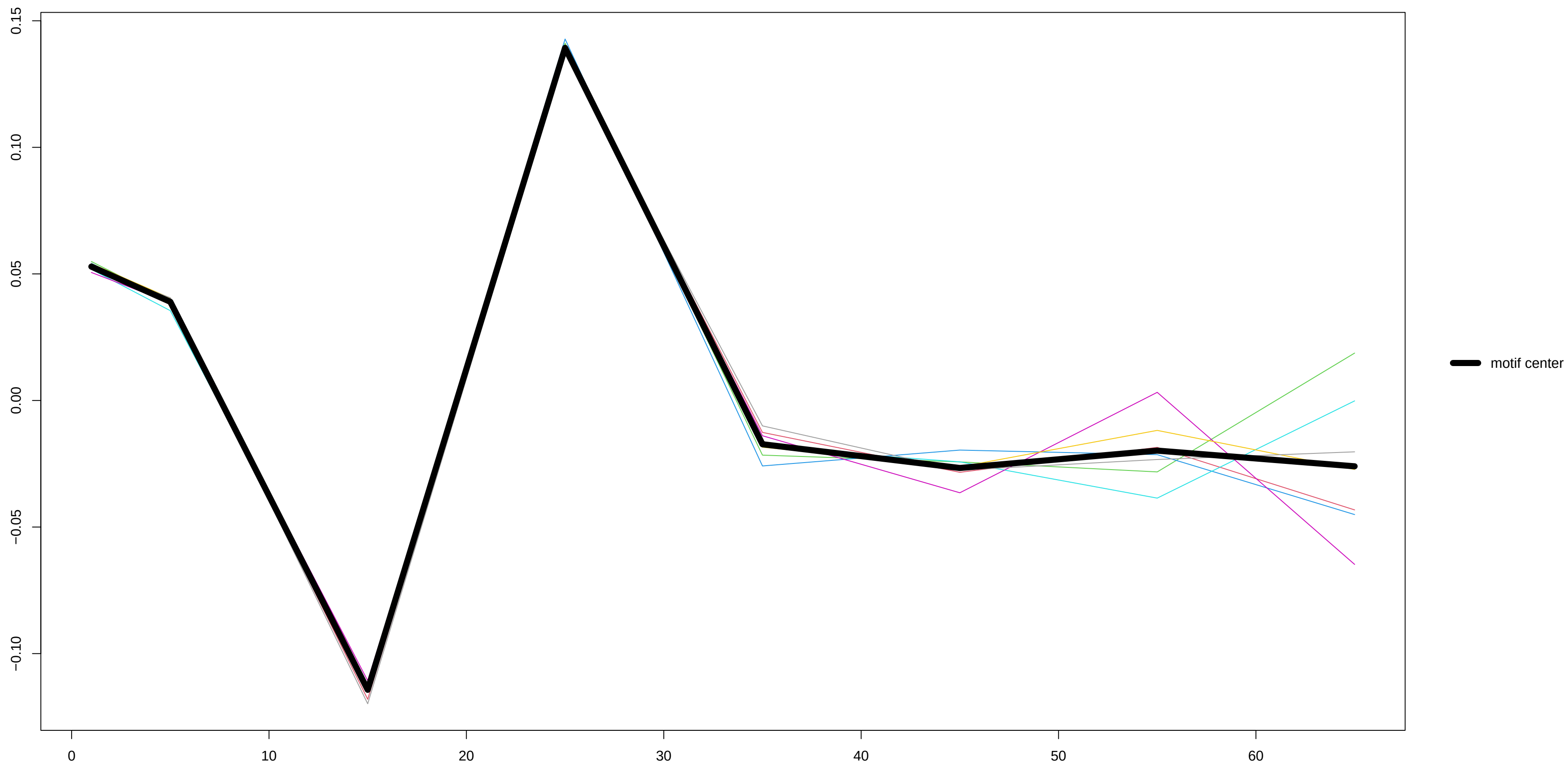
Motif 2 – derivative
