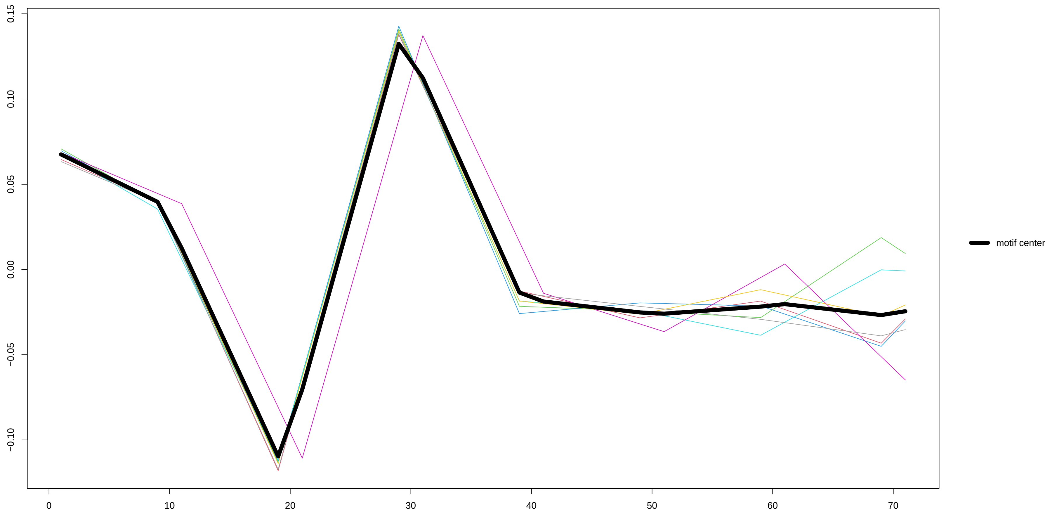
Motif 1 – derivative
