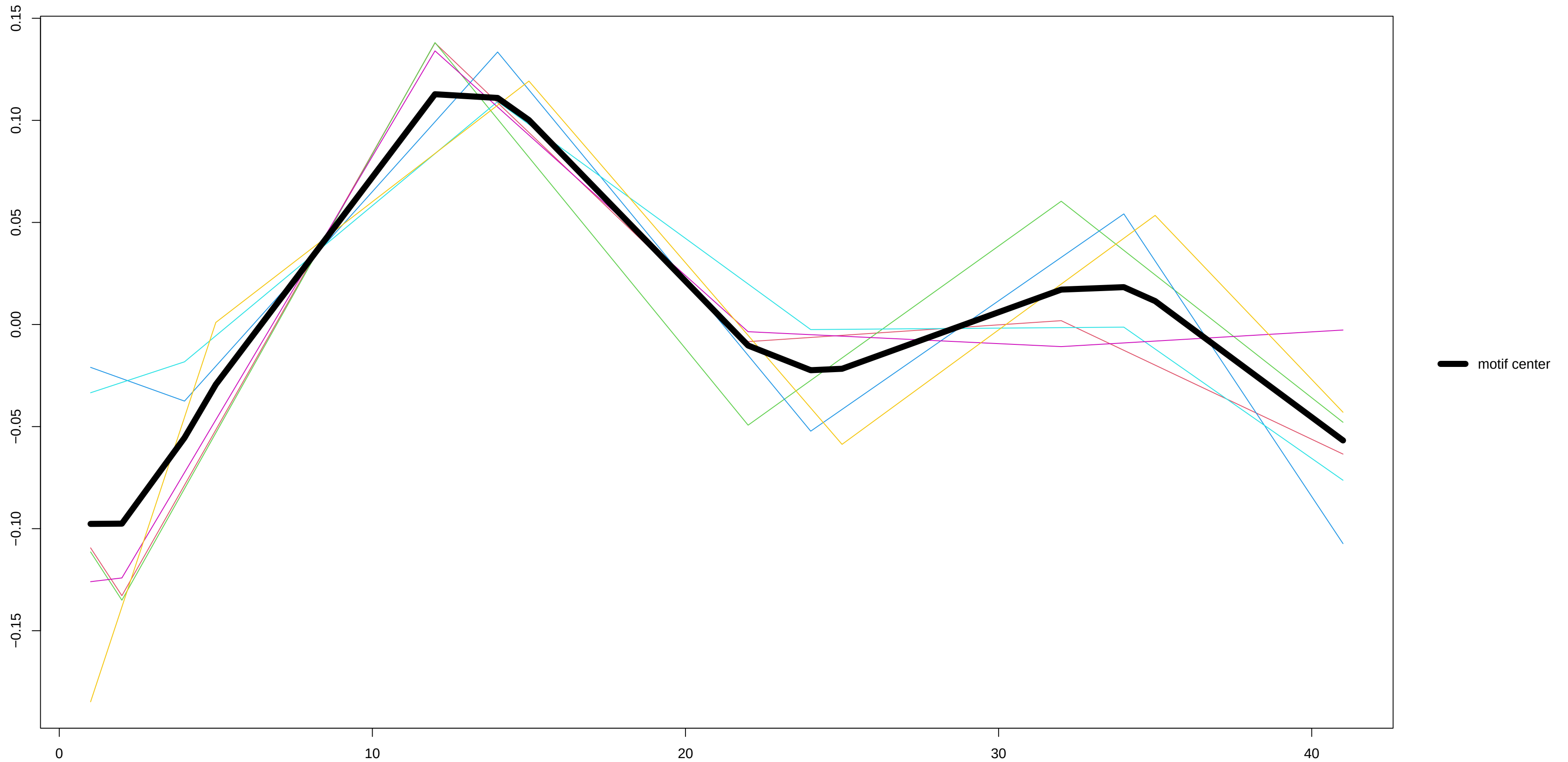
Motif 2 – derivative
