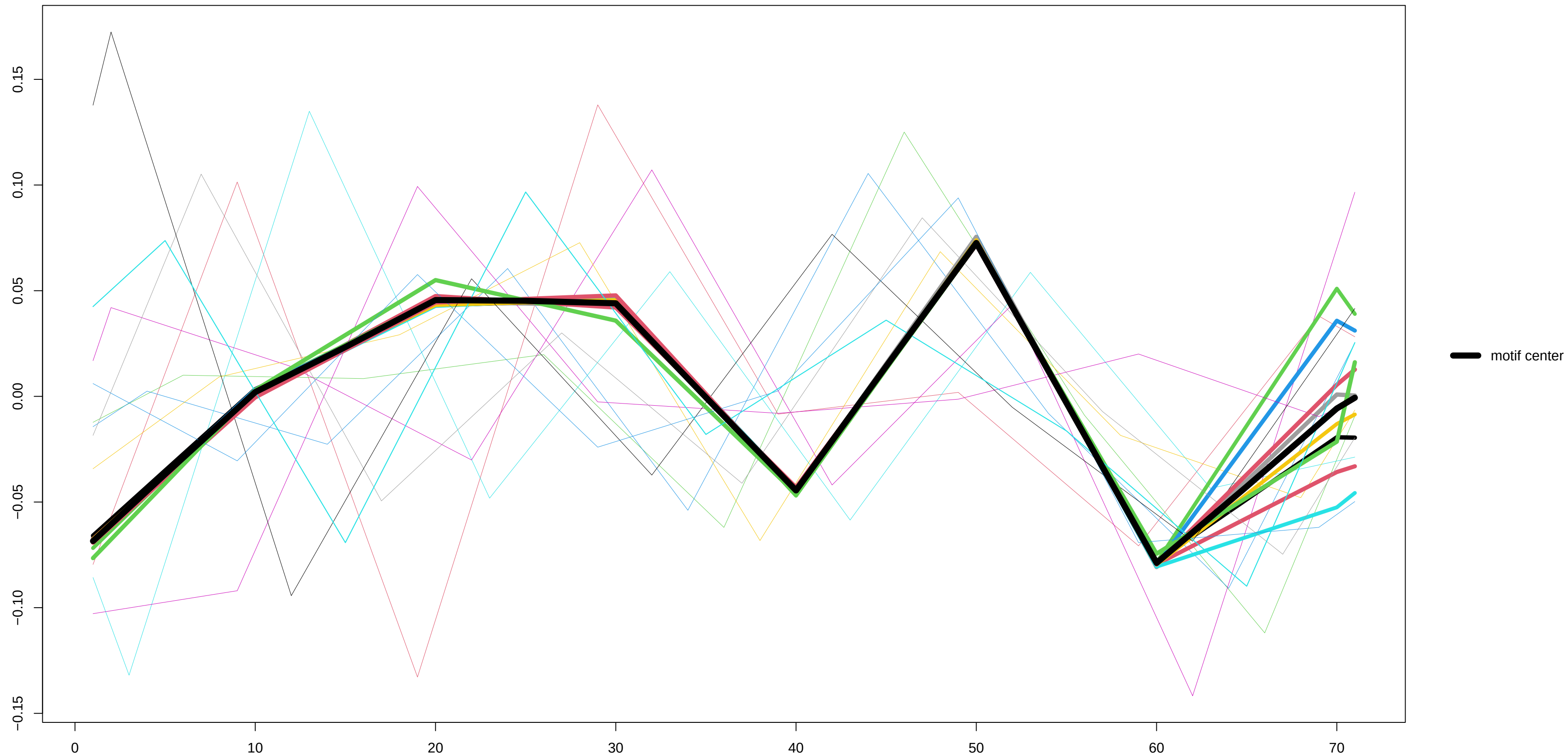
Motif 3 – derivative
