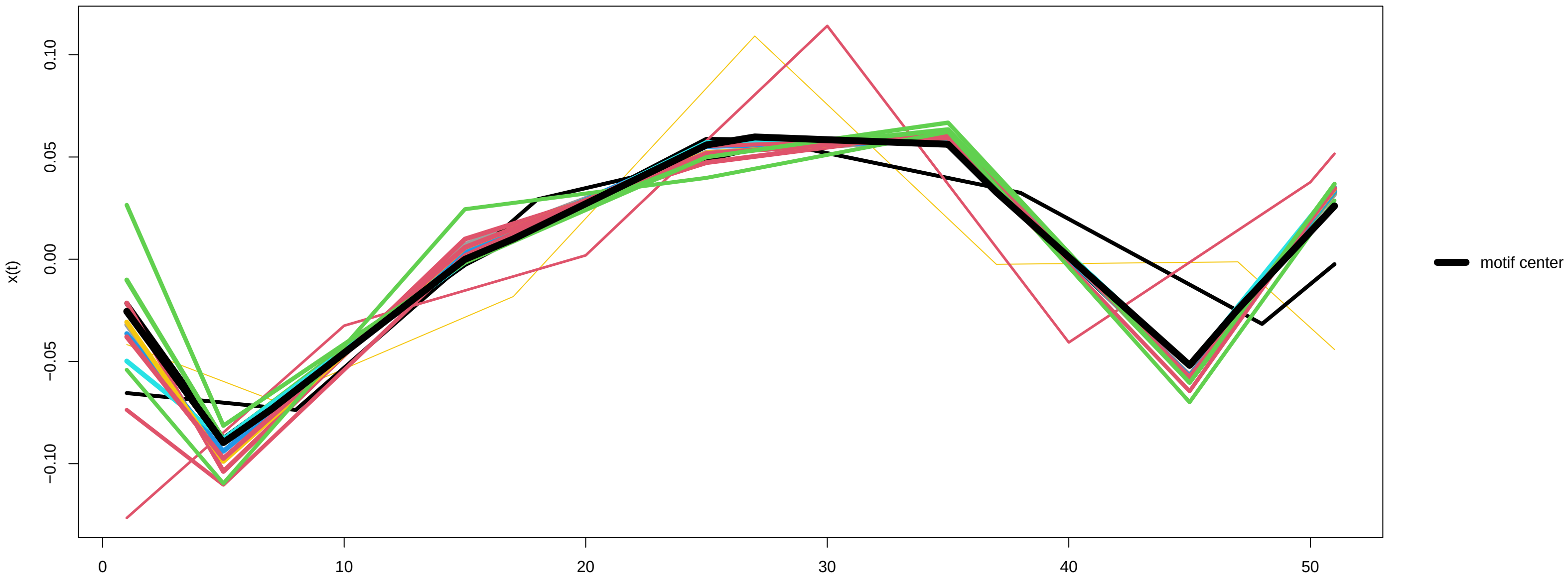
Motif 3 (14 occurrences) – x(t) derivative
