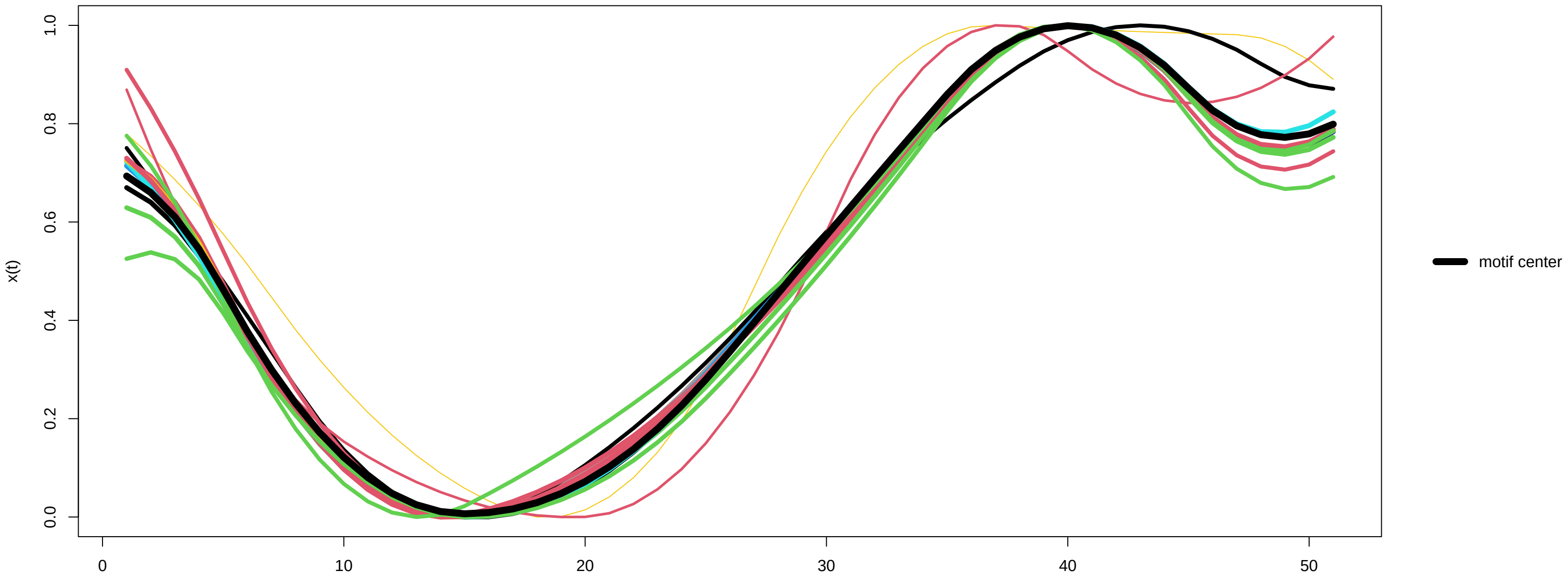
Motif 3 (14 occurrences) – x(t)
