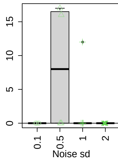
False positives
