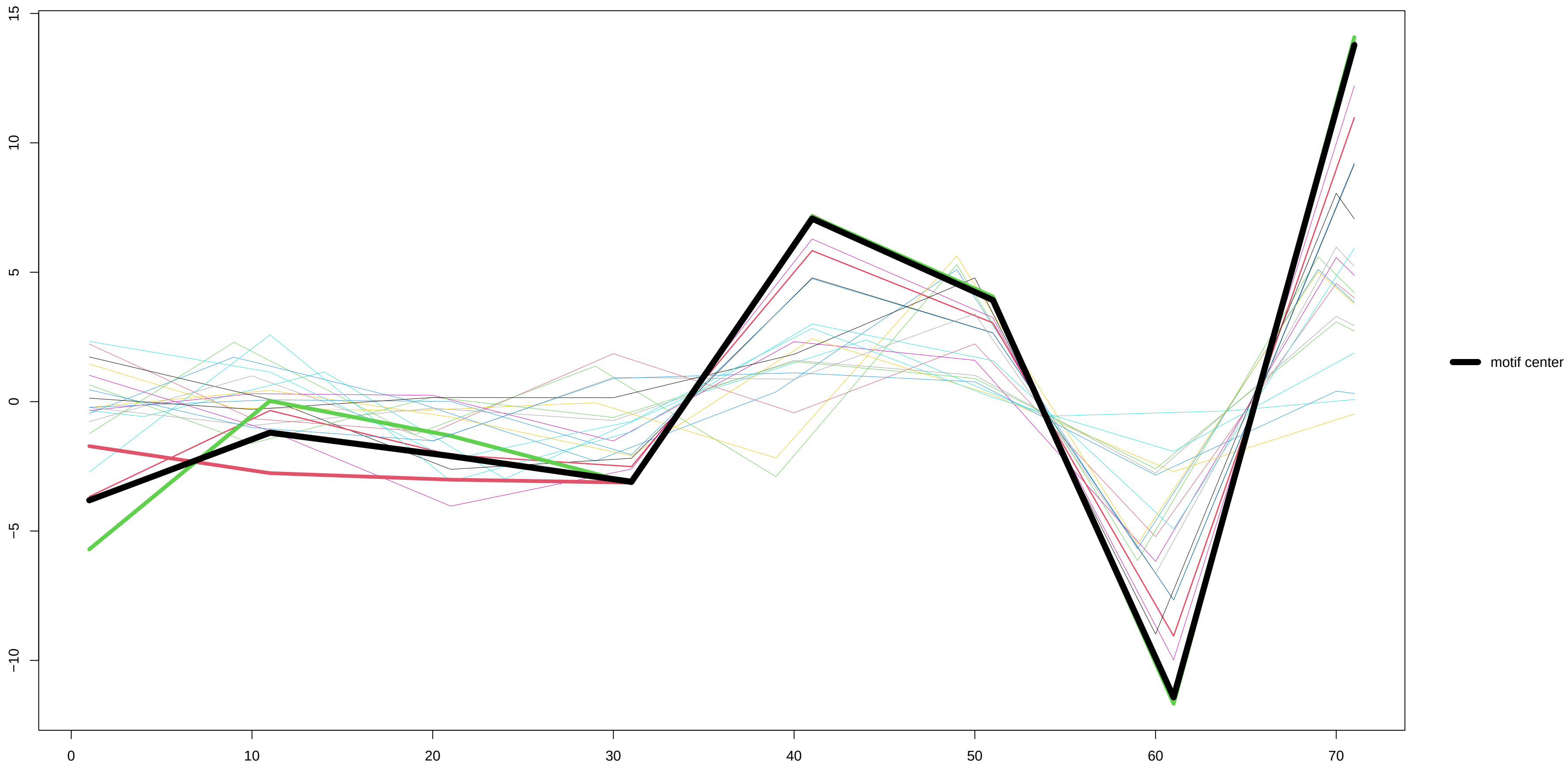
Motif 3 – derivative
