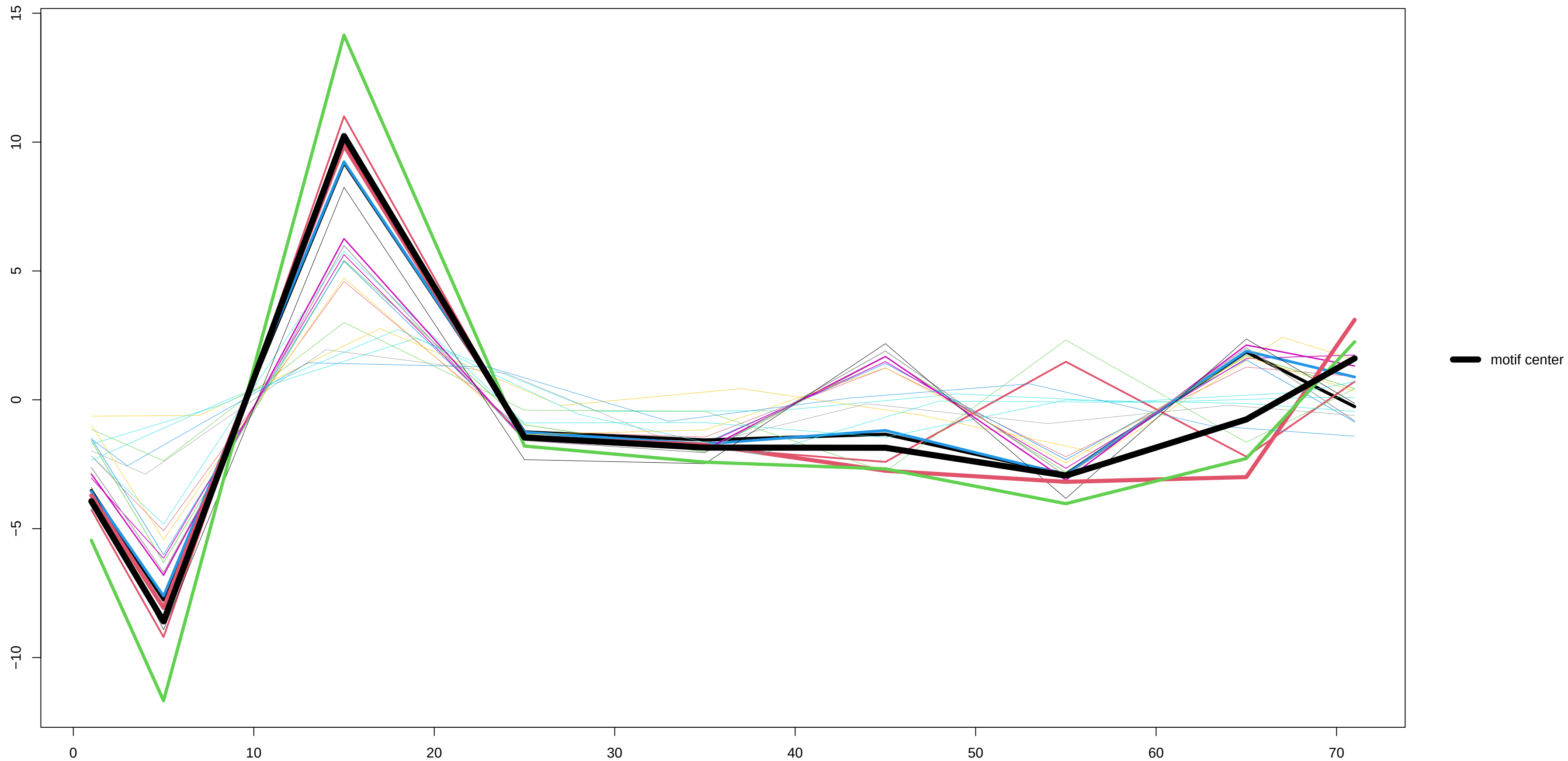
Motif 2 – derivative
