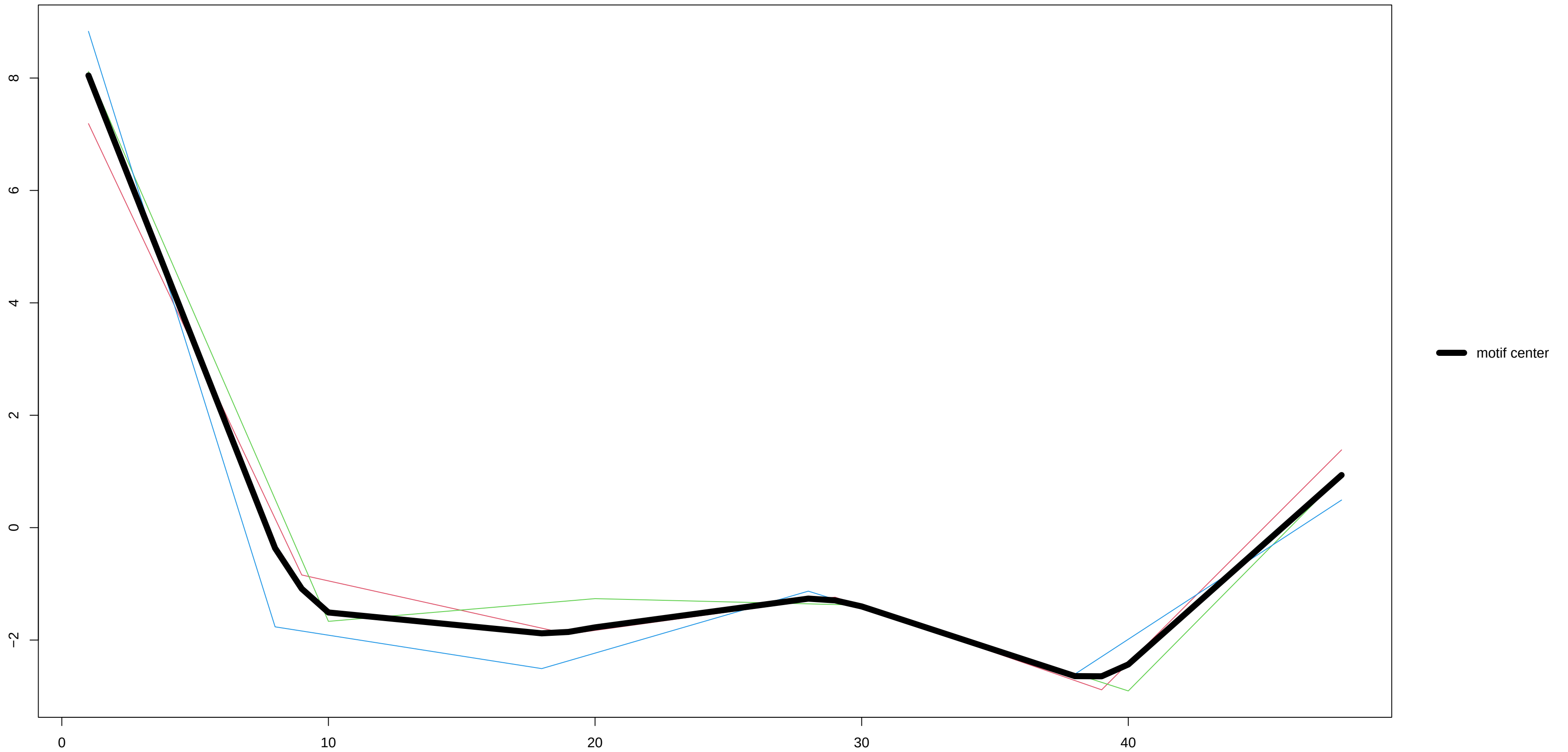
Motif 1 – derivative
