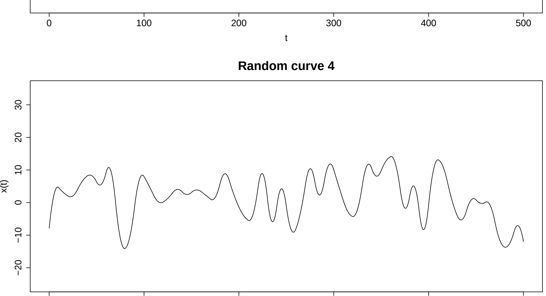
Random curve
