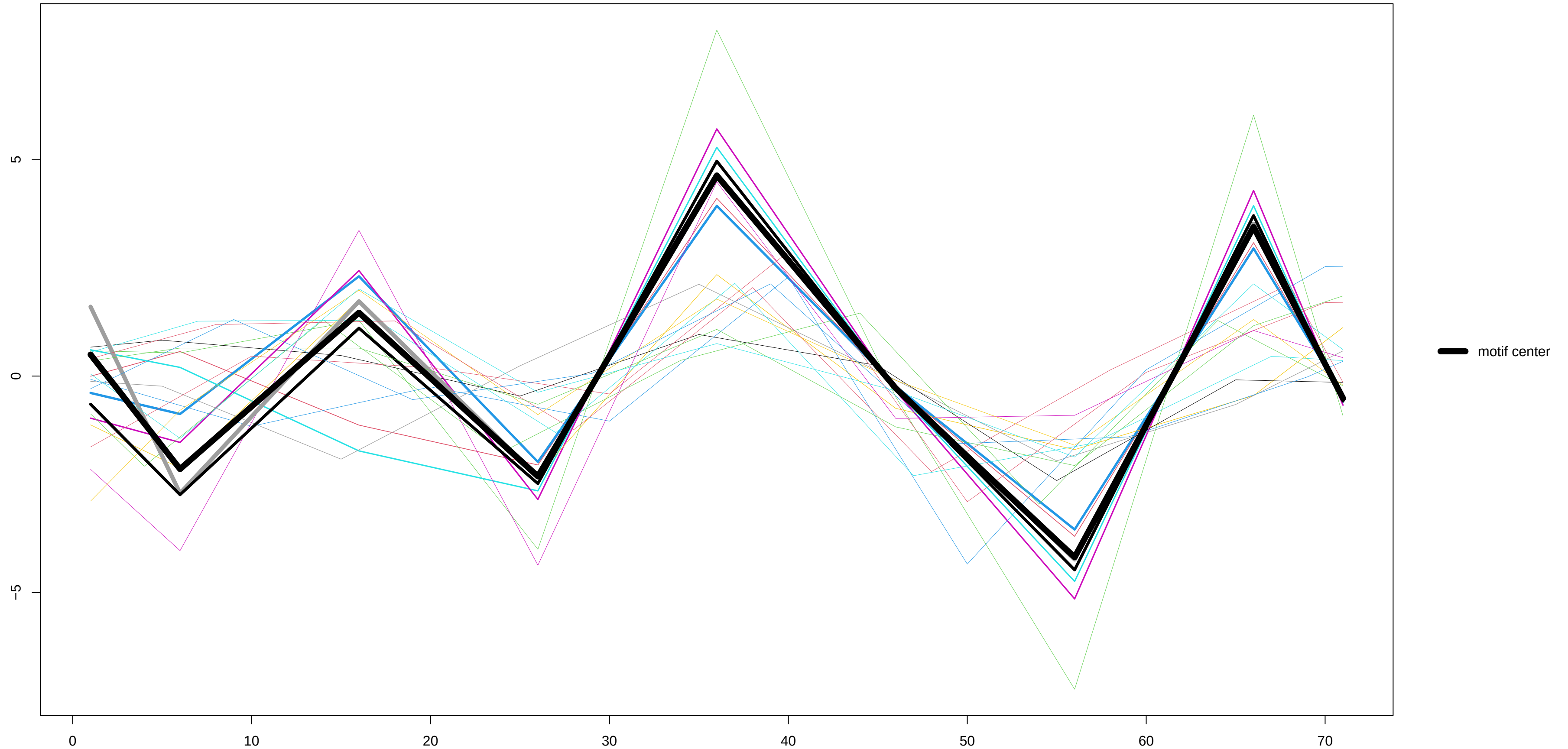
Motif 2 – derivative
