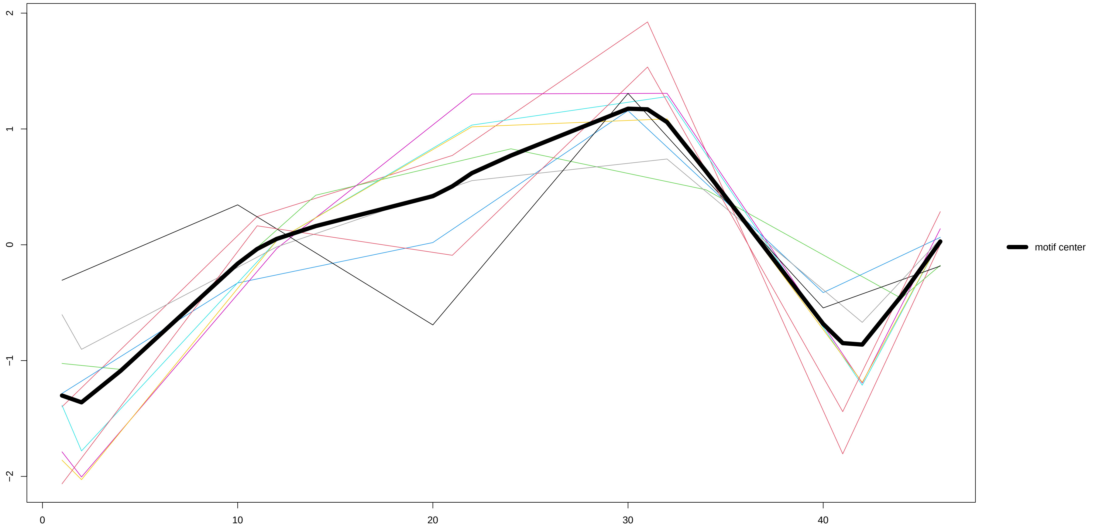
Motif 1 – derivative
