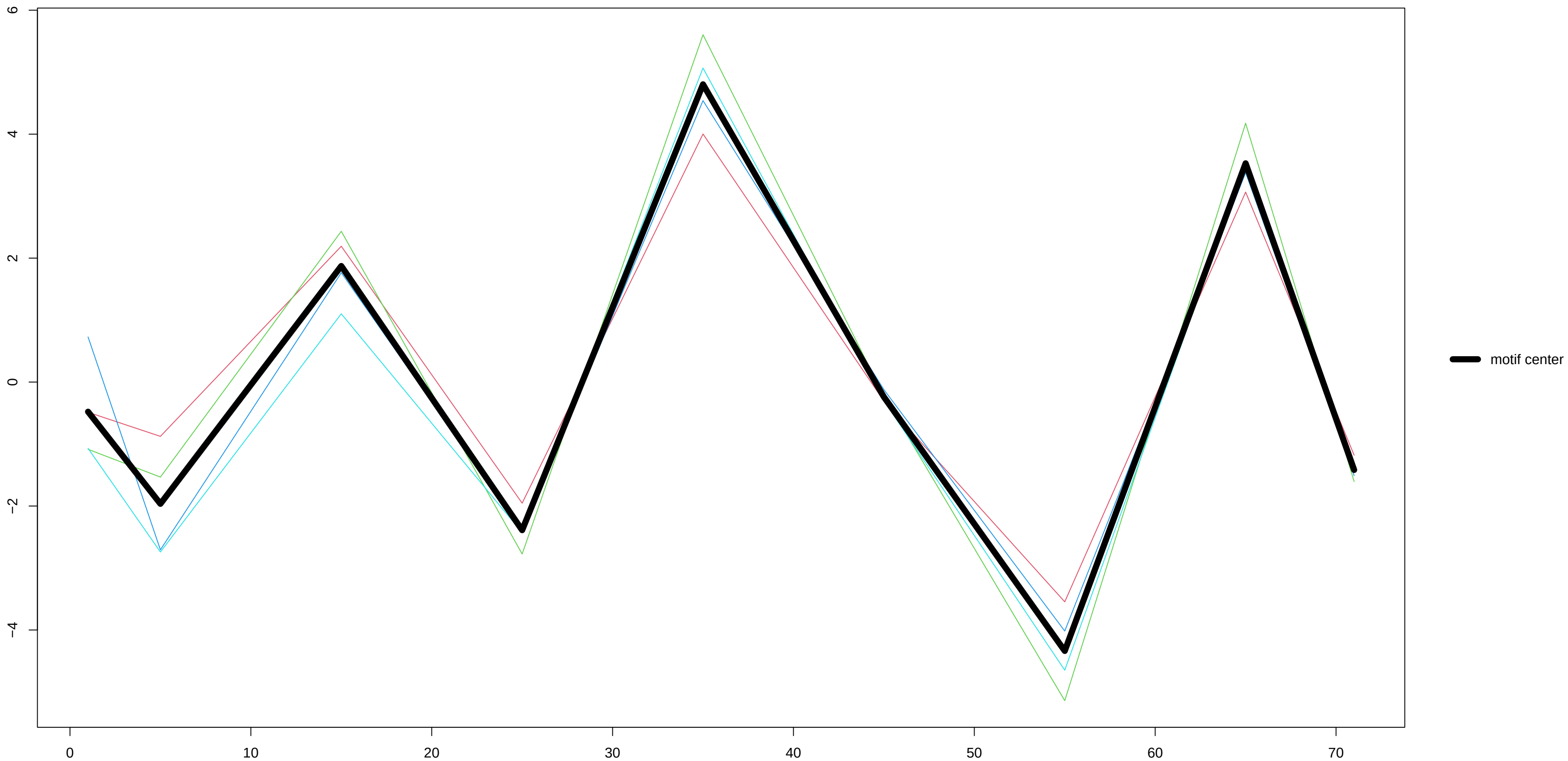
Motif 1 – derivative
