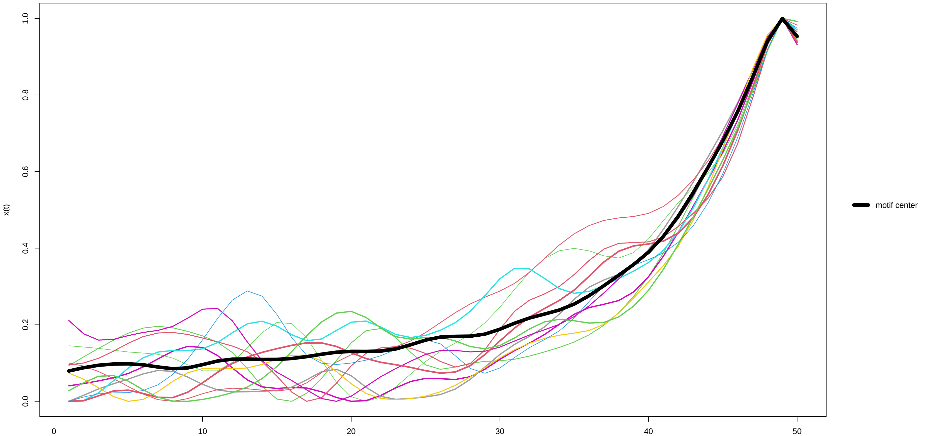
Motif 15 (12 occurrences) – x(t)
