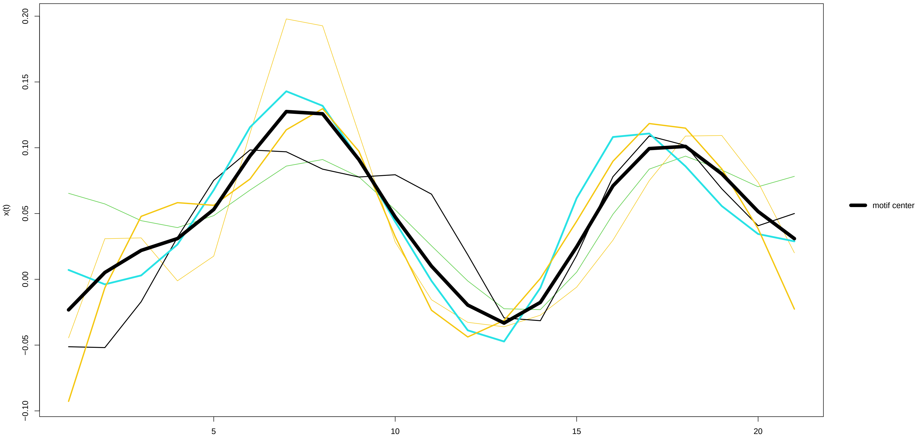
Motif 18 (5 occurrences) – x(t) derivative
