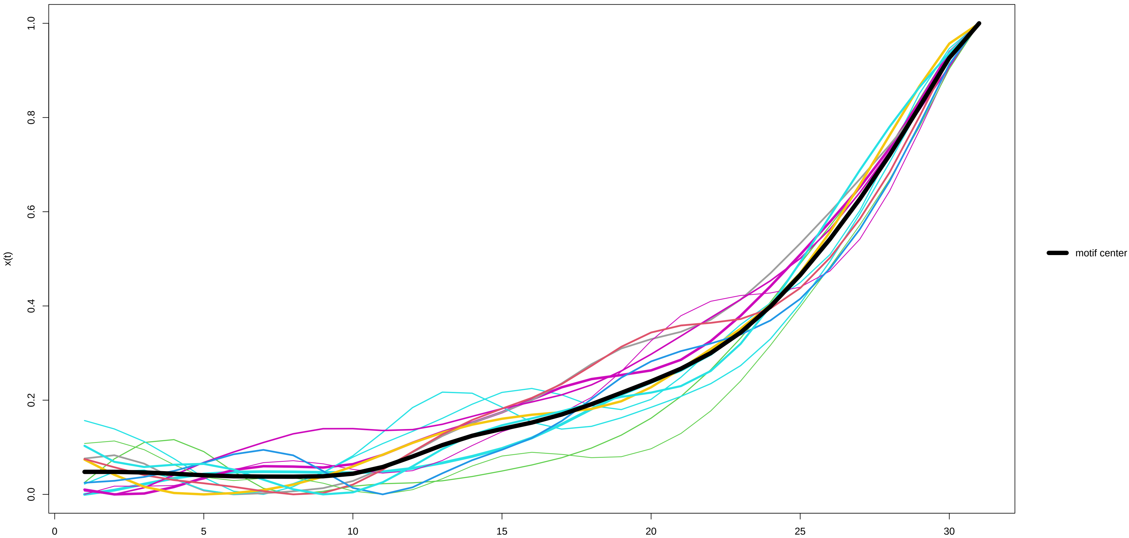
Motif 11 (13 occurrences) – x(t)
