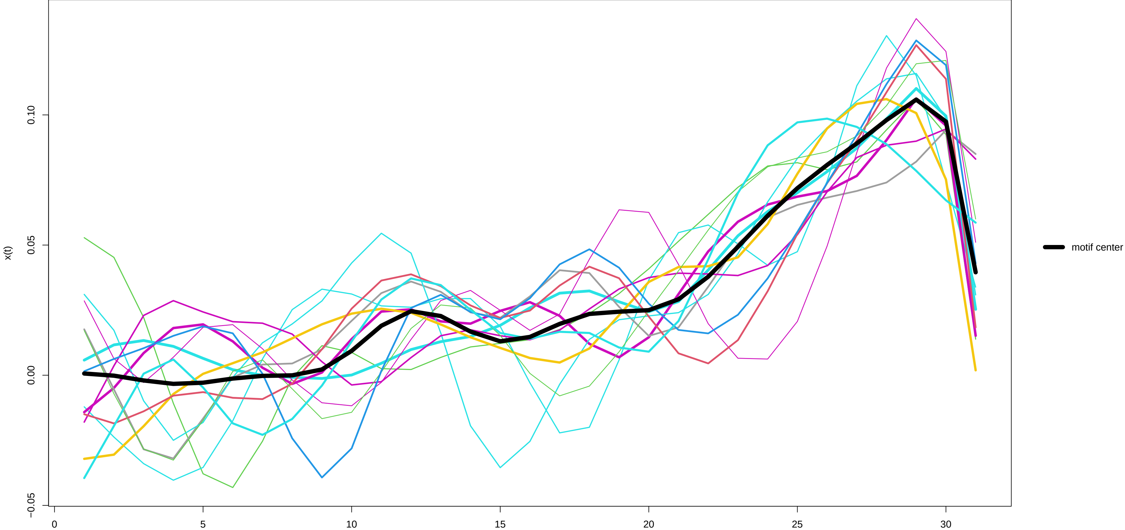
Motif 11 (13 occurrences) – x(t) derivative
