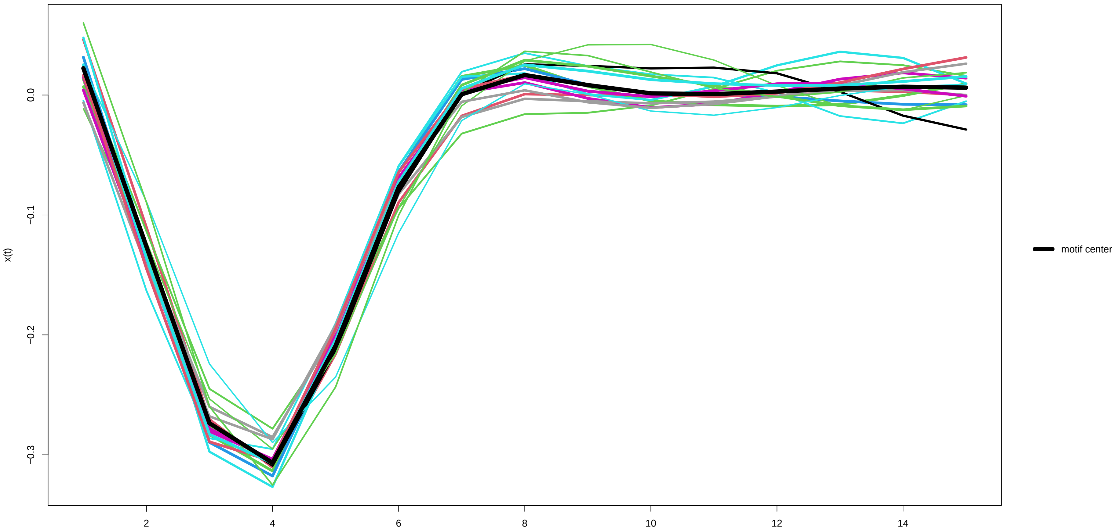
Motif 1 (17 occurrences) – x(t) derivative
