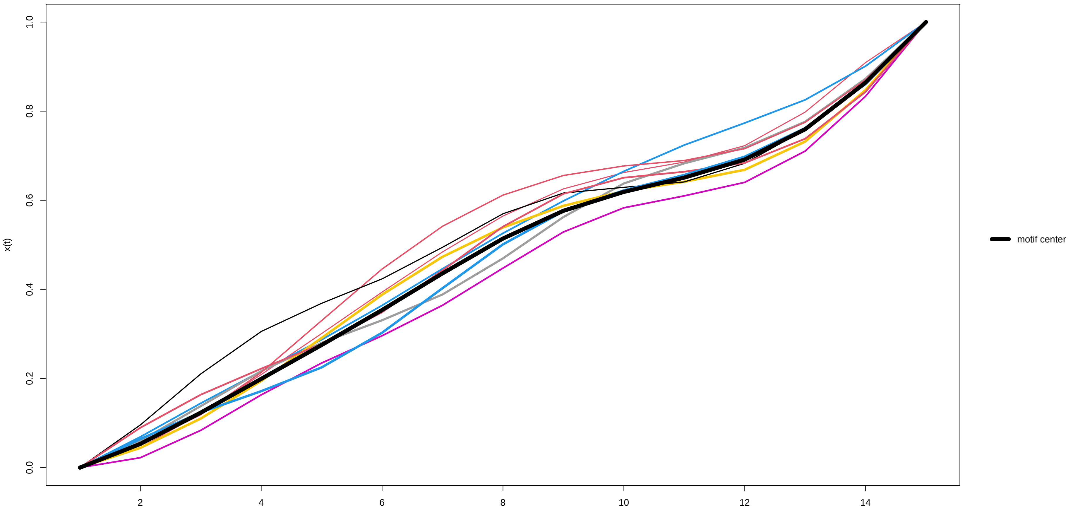
Motif 14 (9 occurrences) – x(t)
