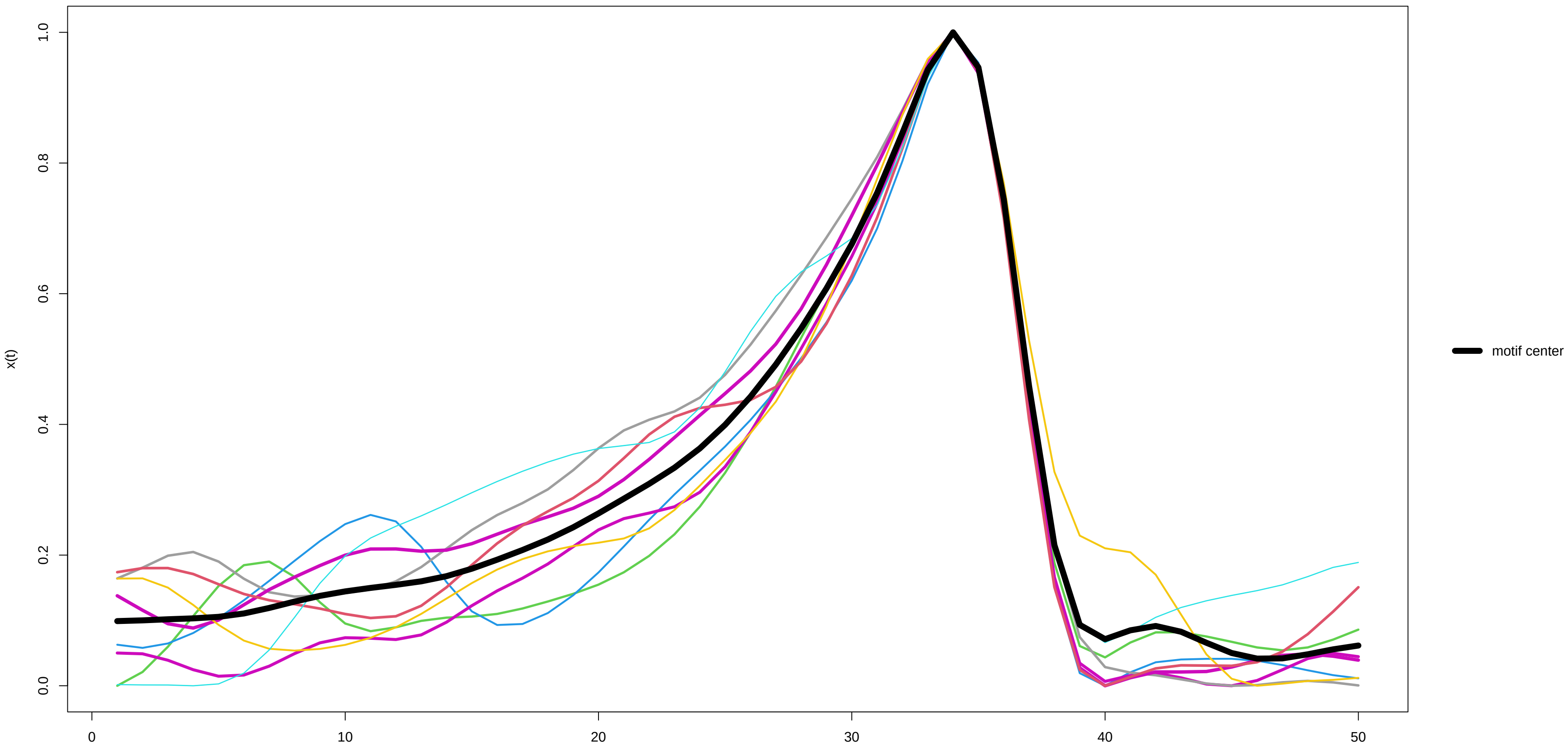
Motif 16 (8 occurrences) – x(t)
