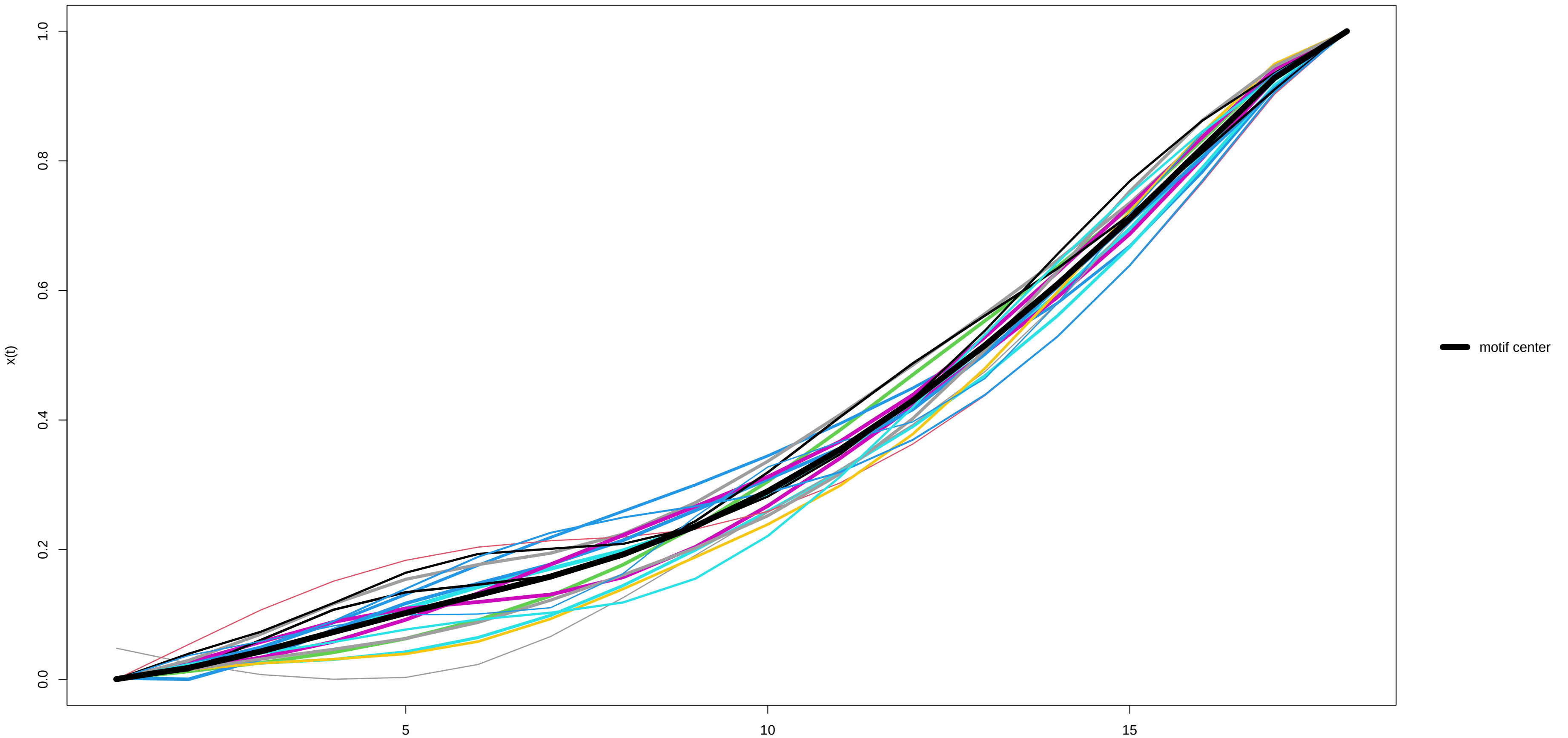
Motif 4 (17 occurrences) – x(t)
