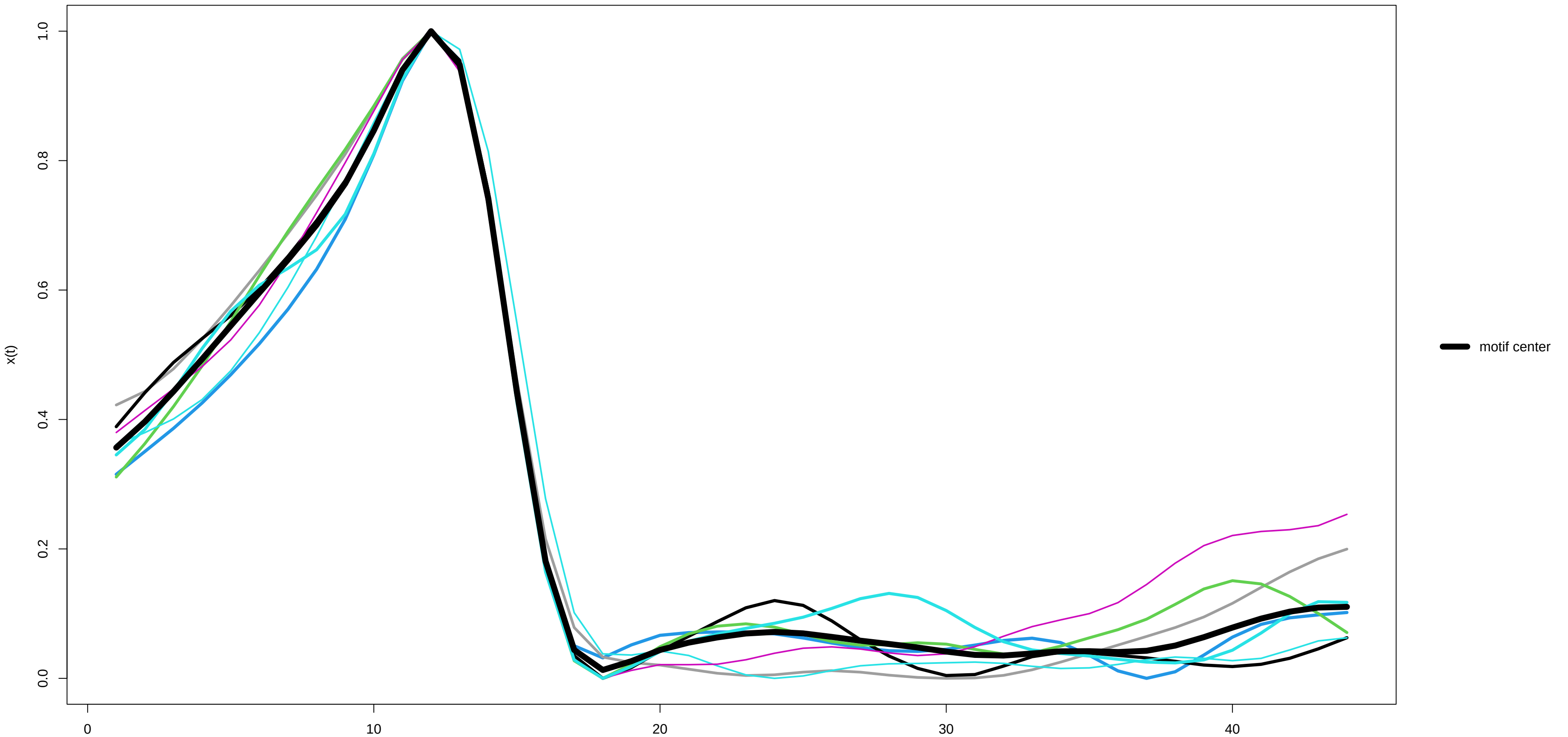
Motif 12 (7 occurrences) – x(t)
