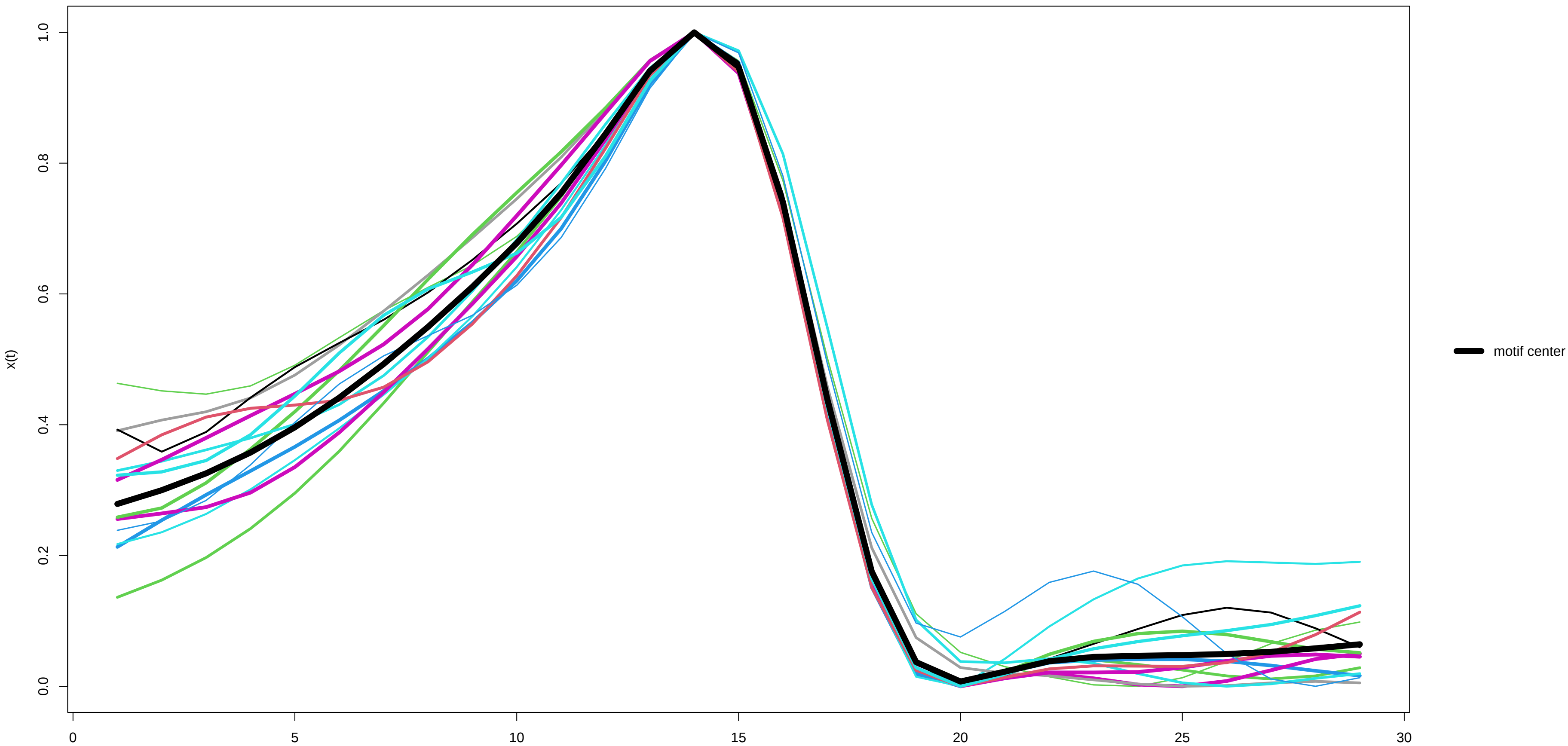
Motif 10 (13 occurrences) – x(t)
