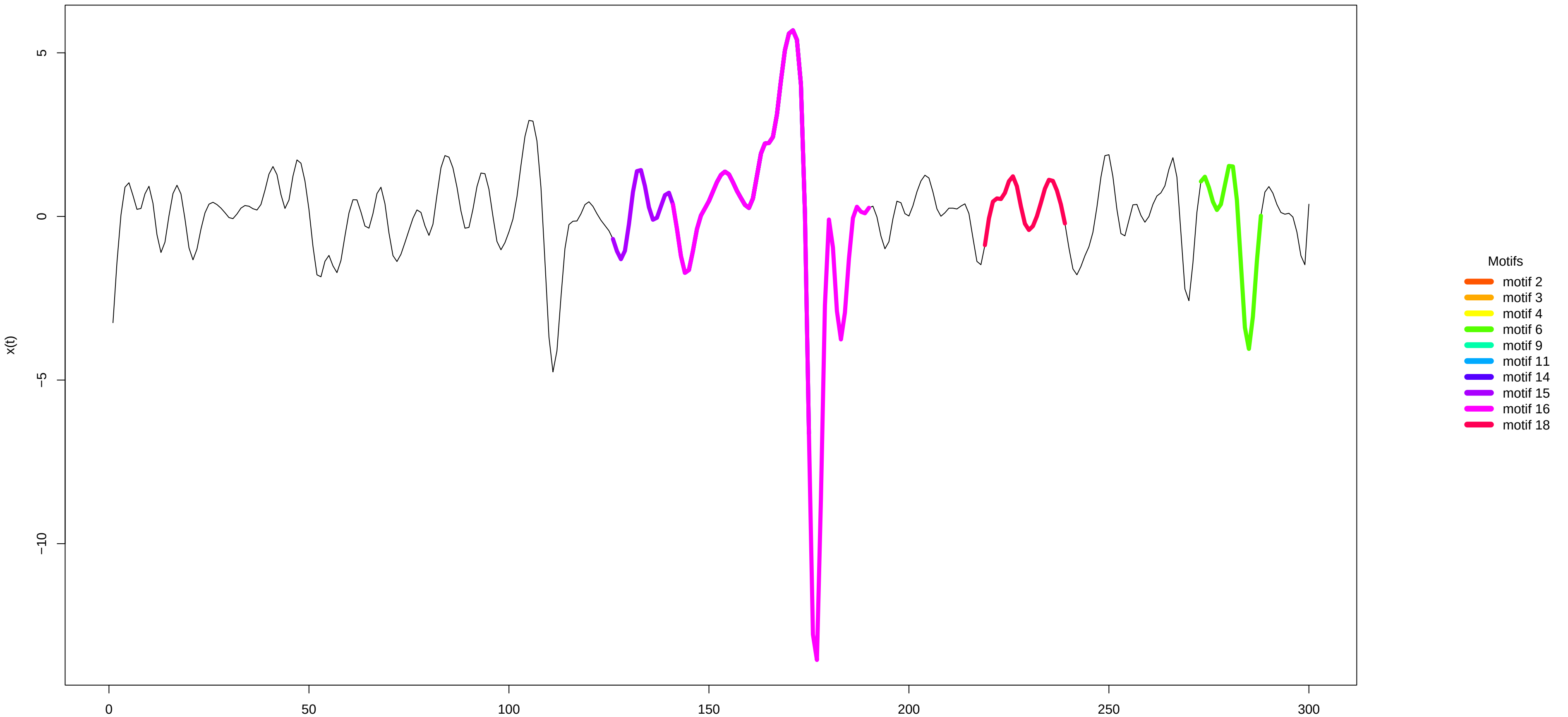
Curve 14 – x(t) derivative
