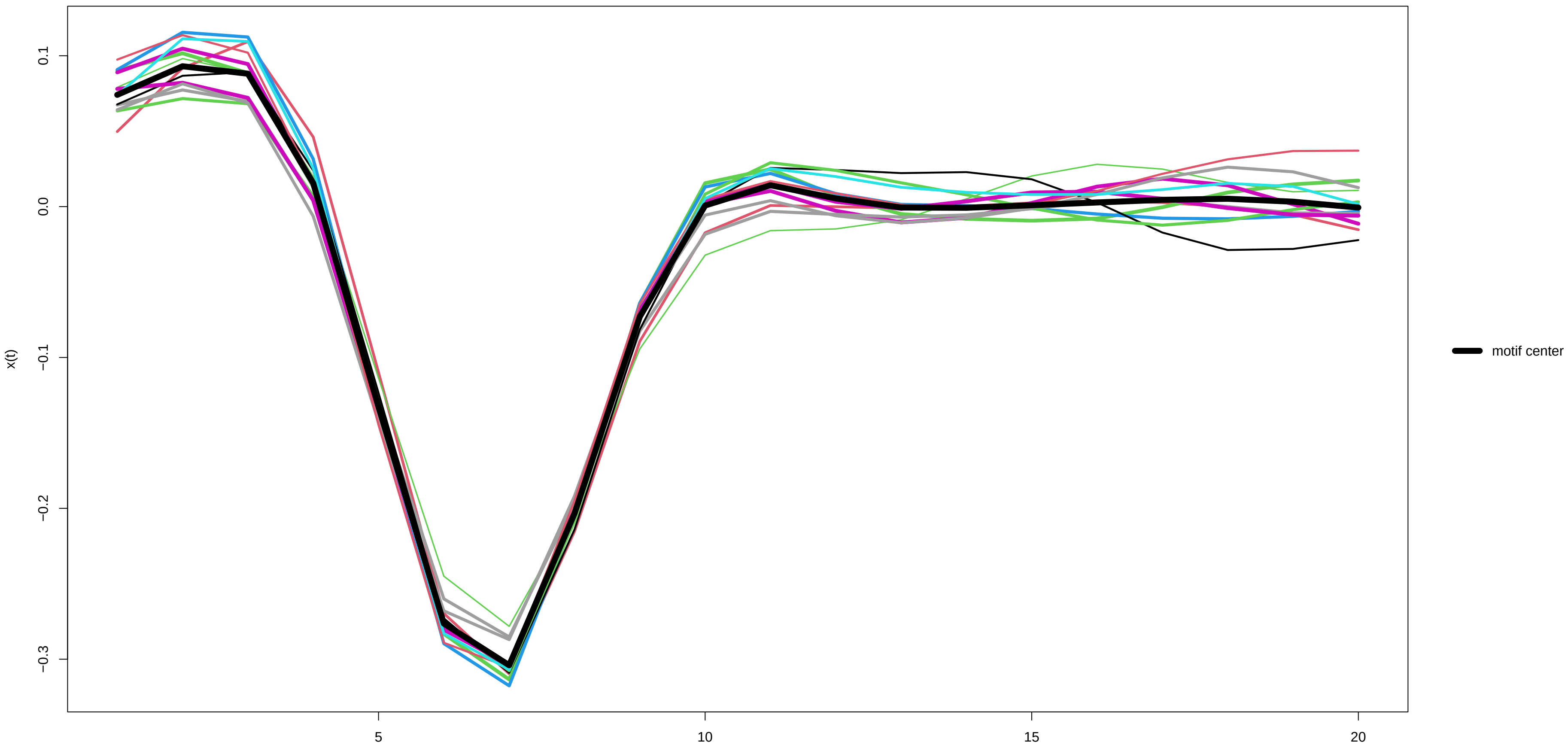
Motif 5 (12 occurrences) – x(t) derivative
