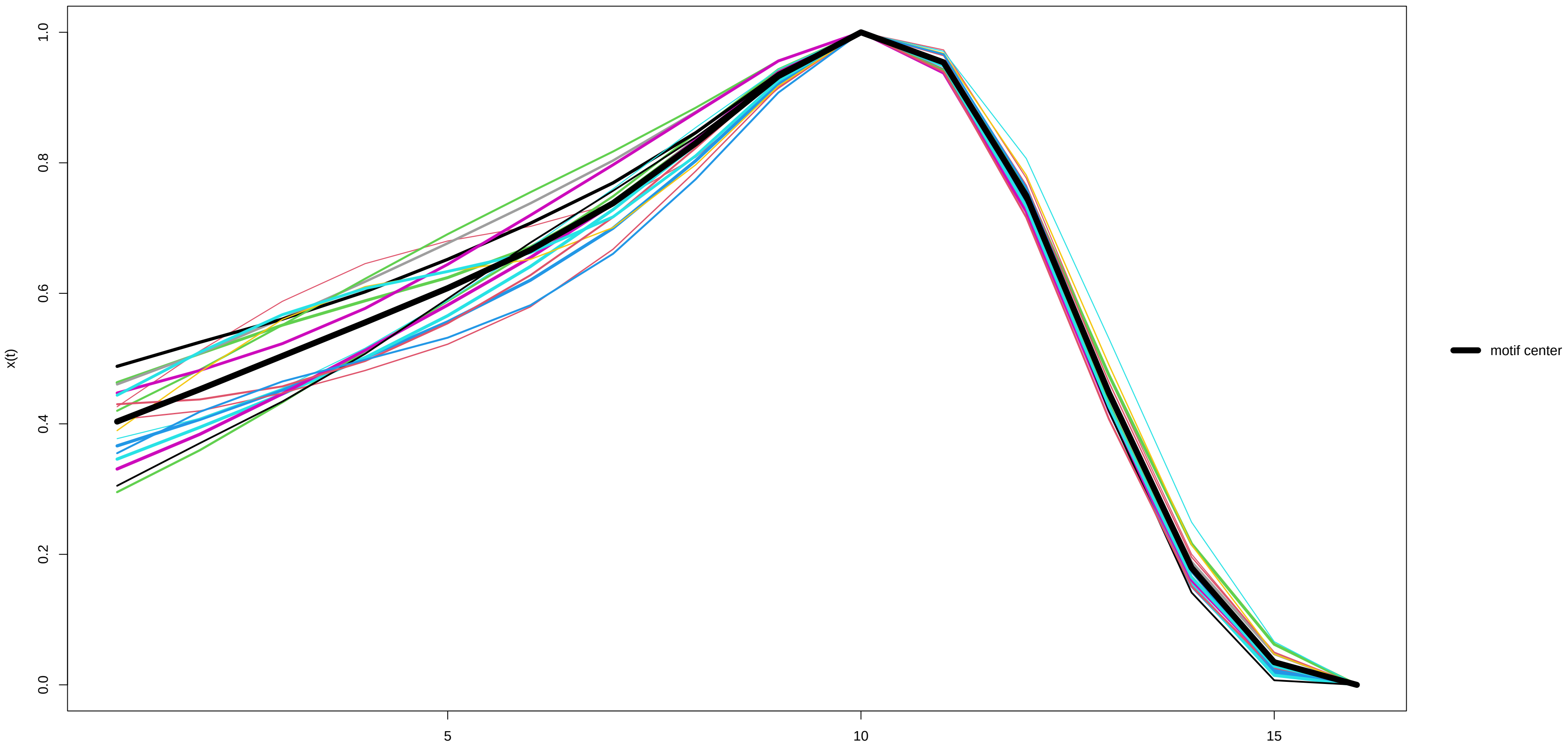
Motif 6 (17 occurrences) – x(t)
