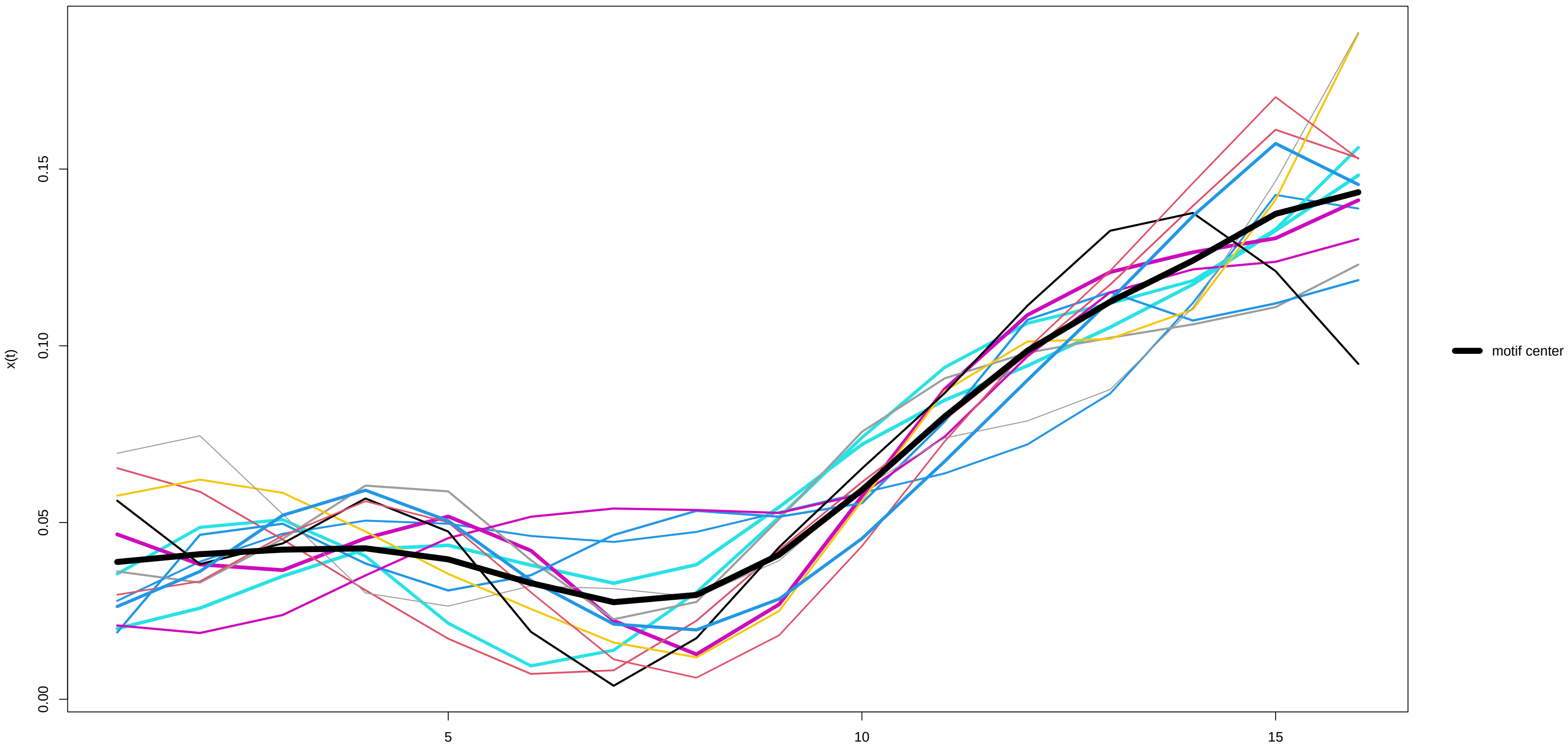
Motif 3 (13 occurrences) – x(t) derivative
