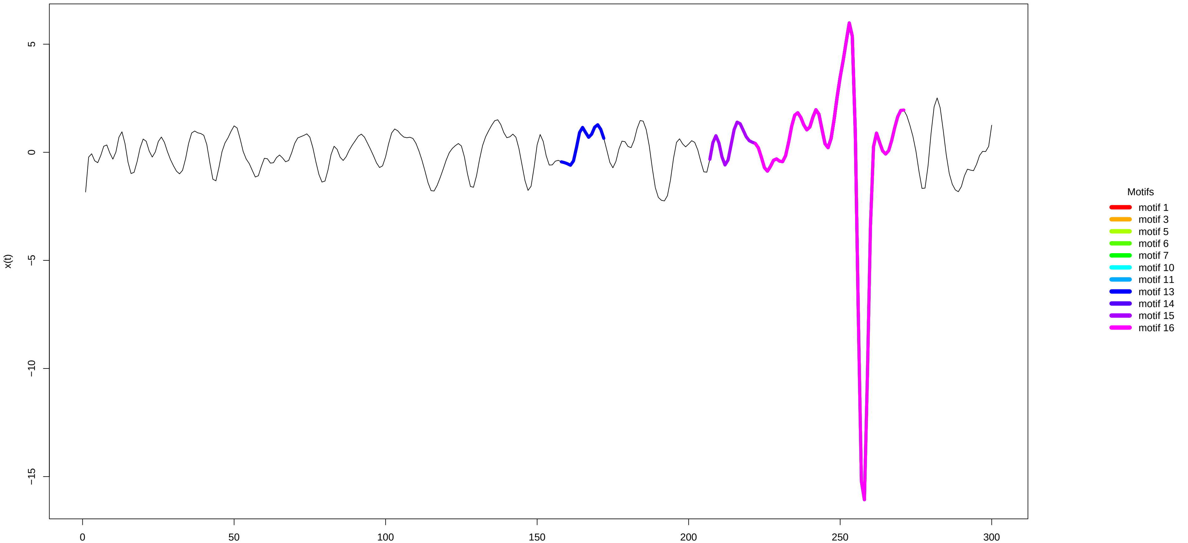
Curve 17 – x(t) derivative
