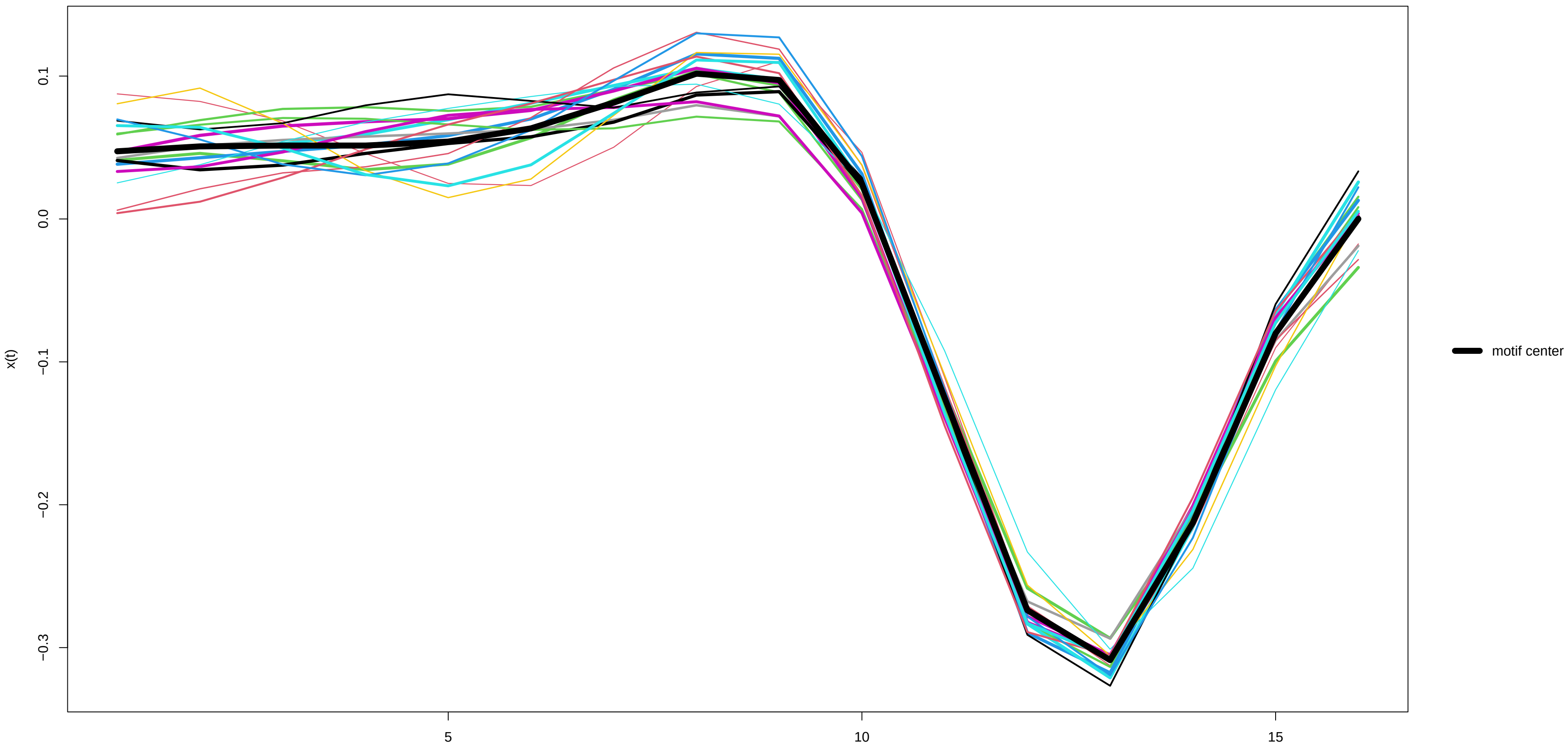
Motif 6 (17 occurrences) – x(t) derivative
