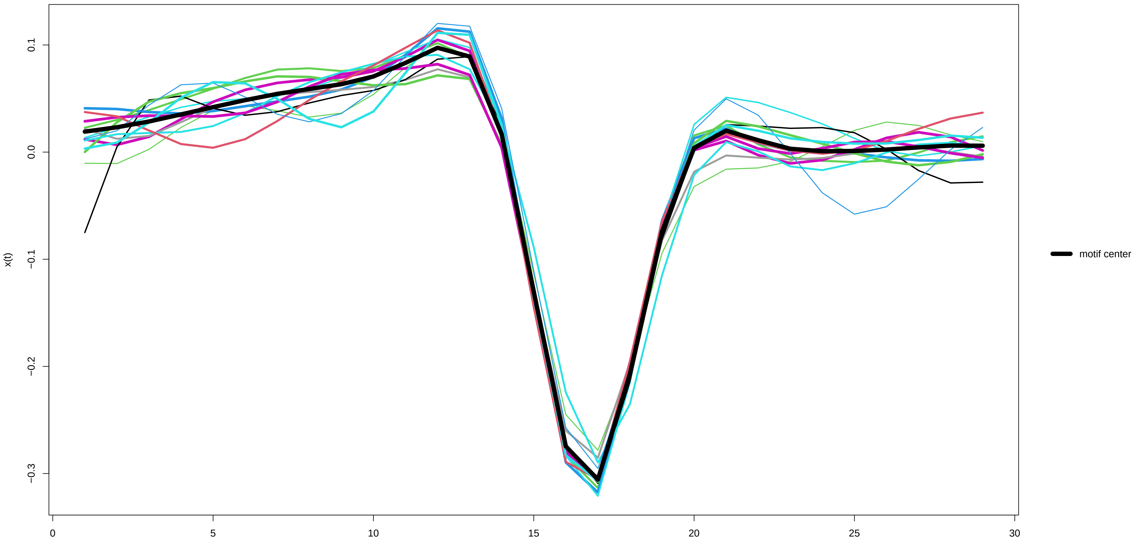
Motif 10 (13 occurrences) – x(t) derivative
