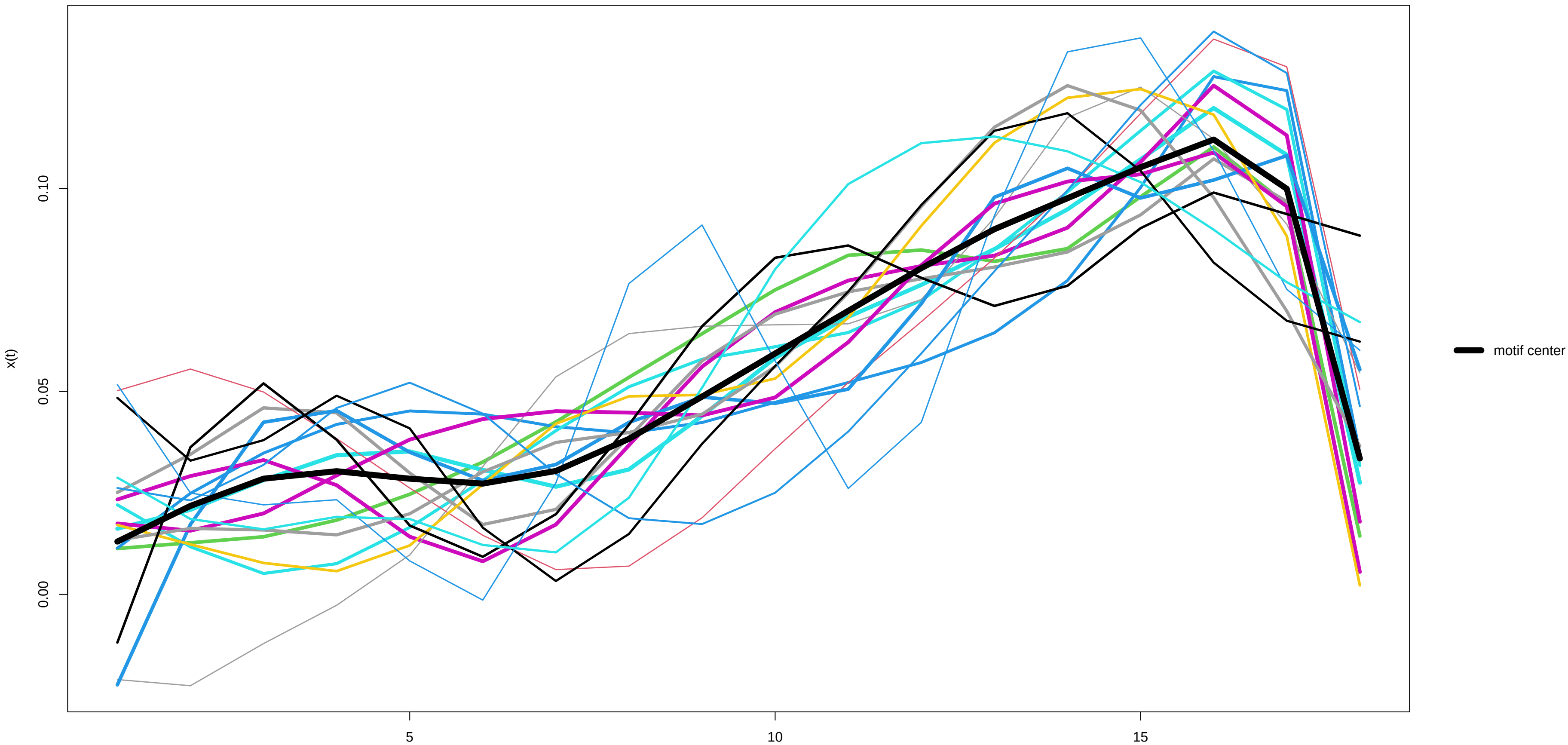
Motif 4 (17 occurrences) – x(t) derivative
