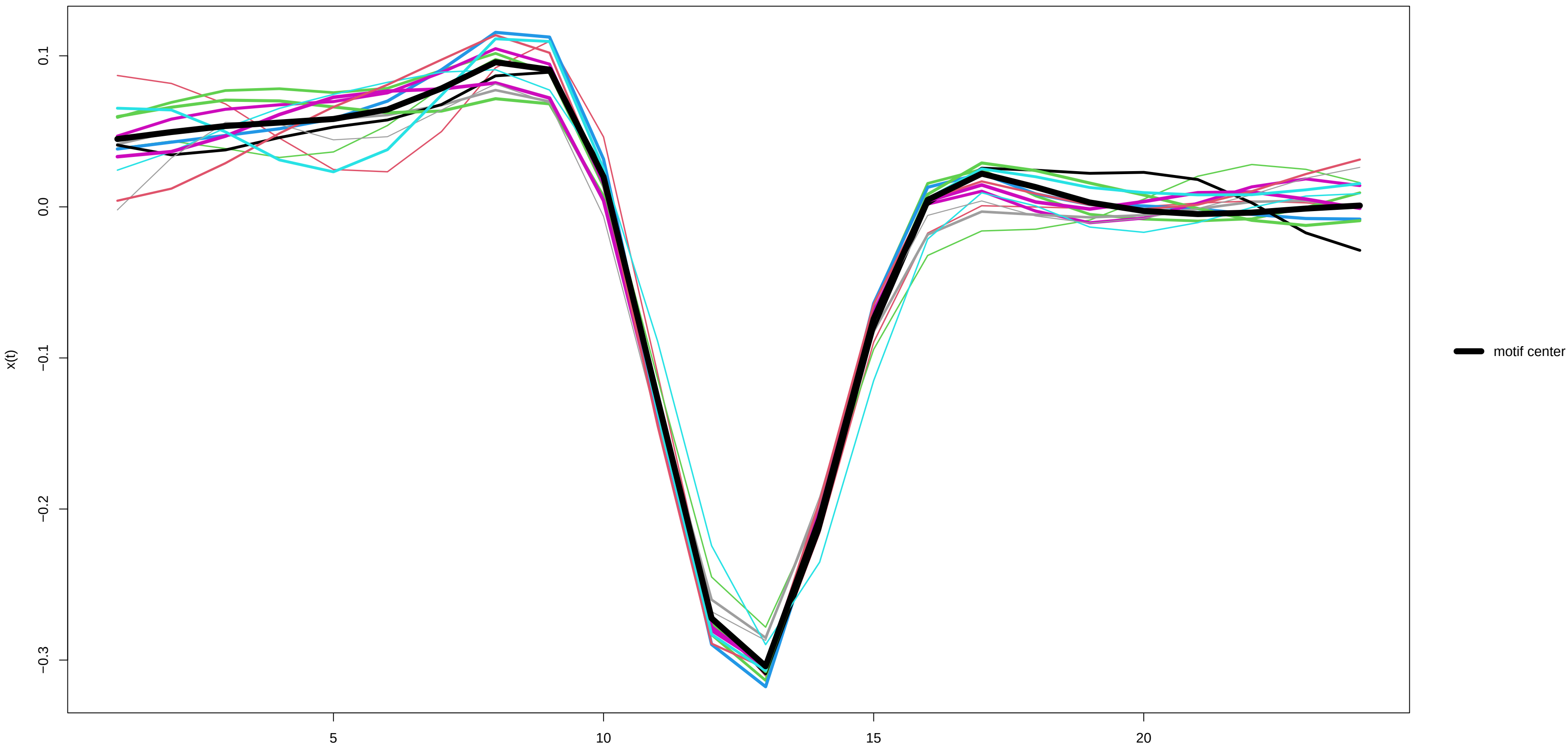
Motif 7 (13 occurrences) – x(t) derivative
