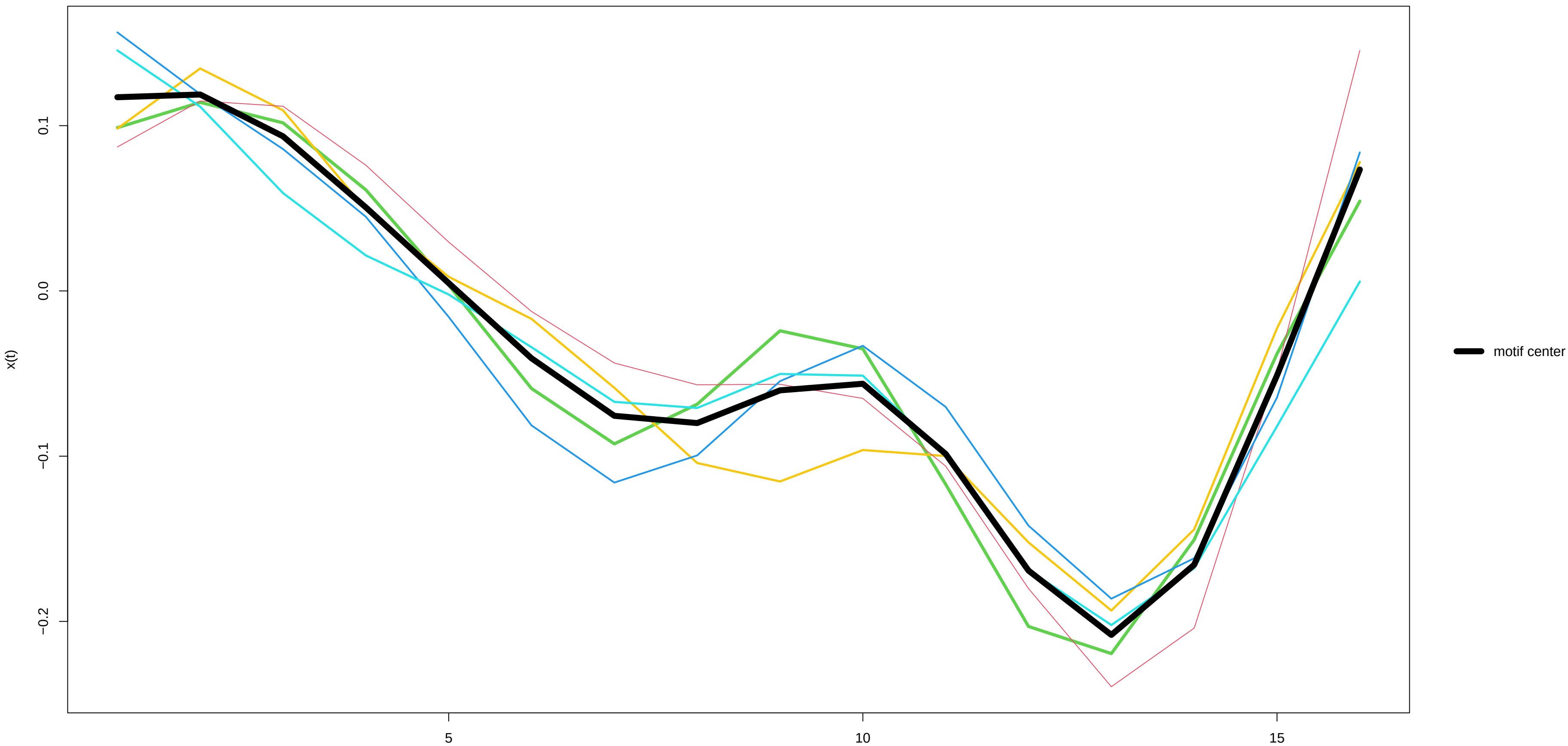
Motif 17 (5 occurrences) – x(t) derivative
