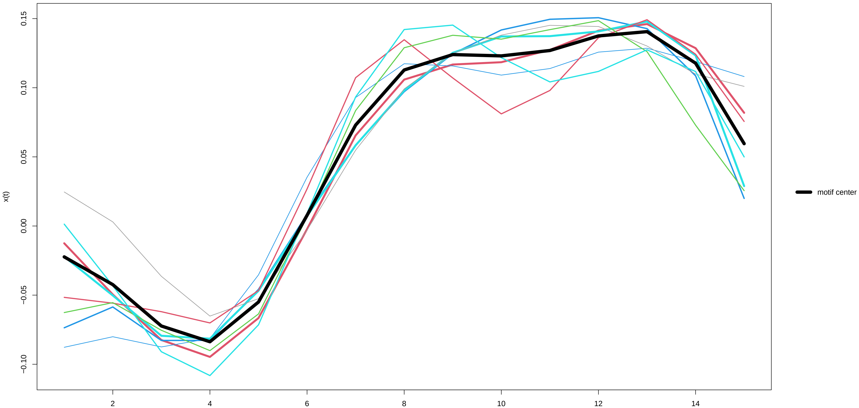
Motif 13 (8 occurrences) – x(t) derivative
