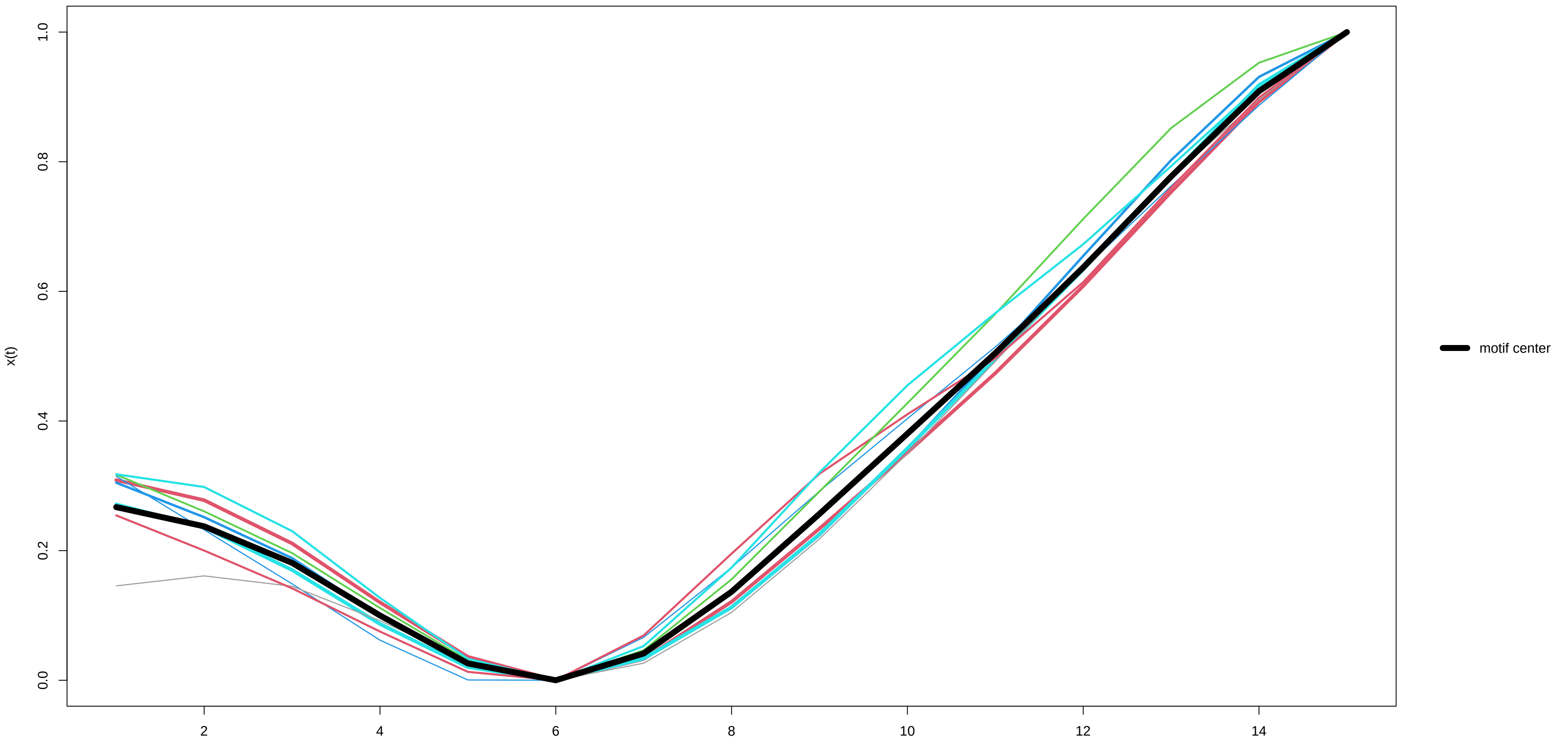
Motif 13 (8 occurrences) – x(t)
