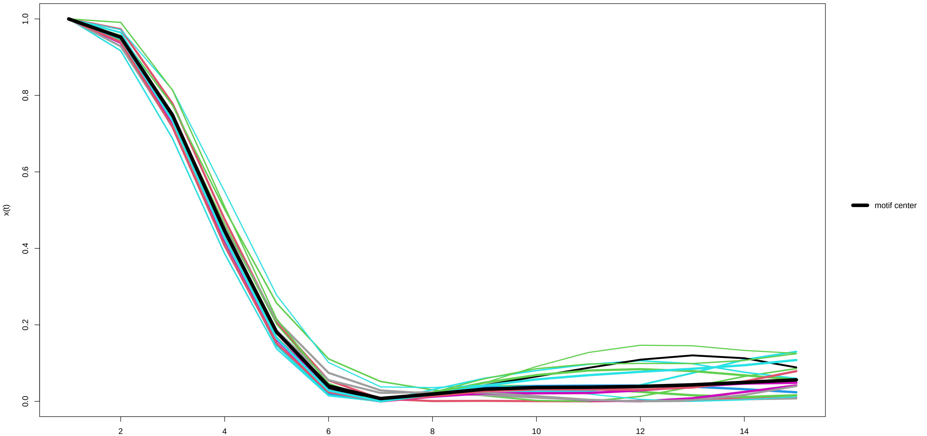
Motif 1 (17 occurrences) – x(t)
