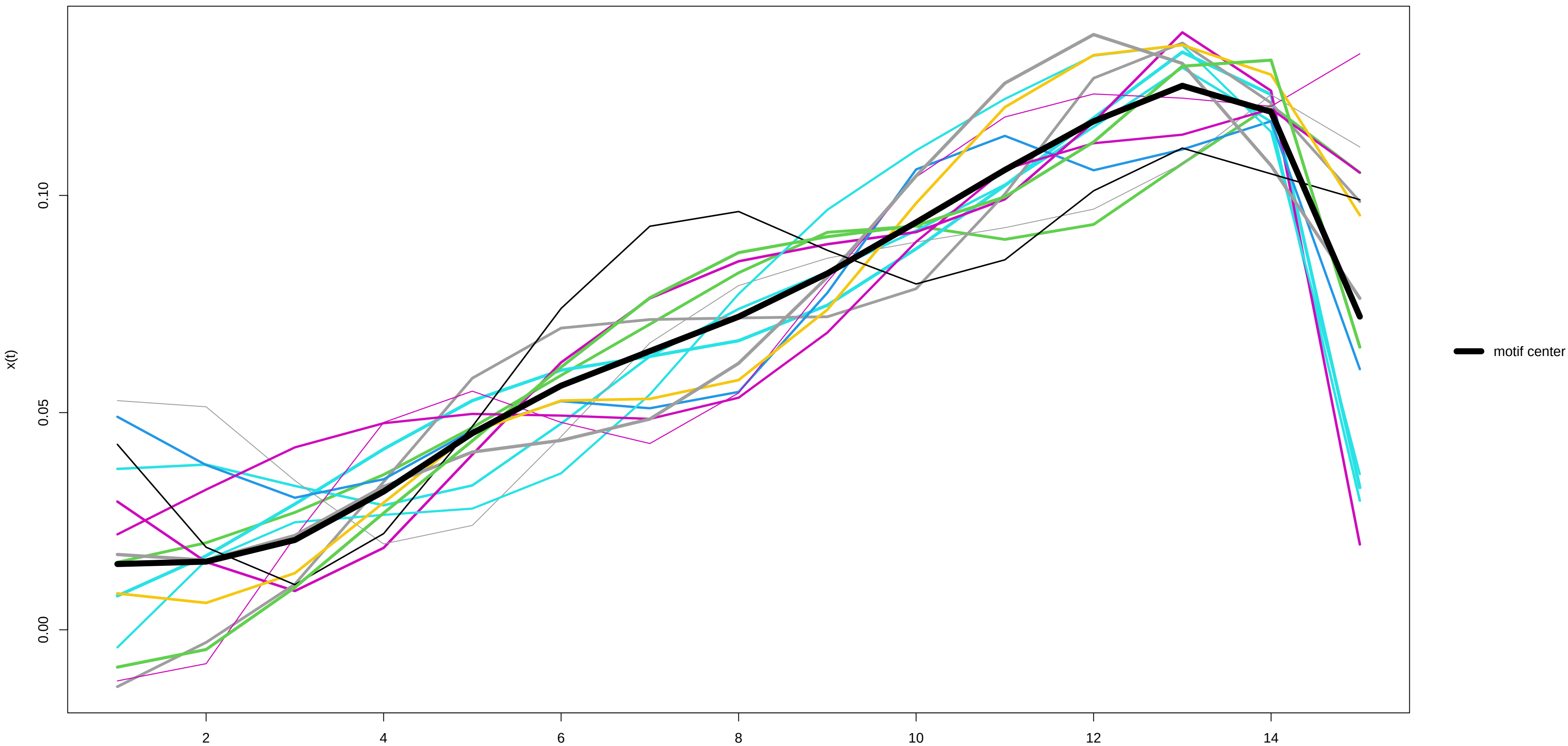
Motif 2 (14 occurrences) – x(t) derivative
