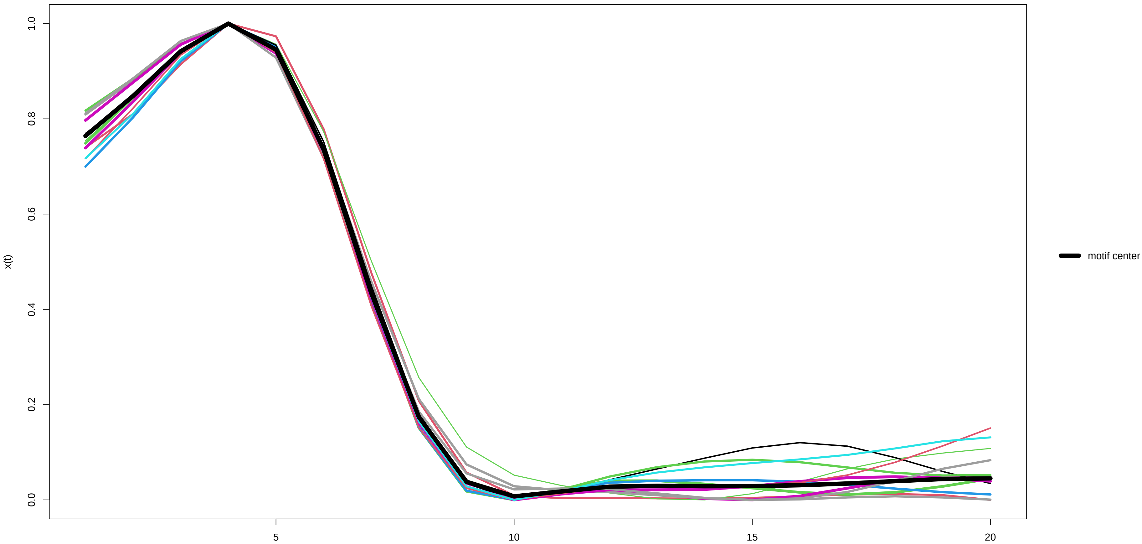
Motif 5 (12 occurrences) – x(t)
