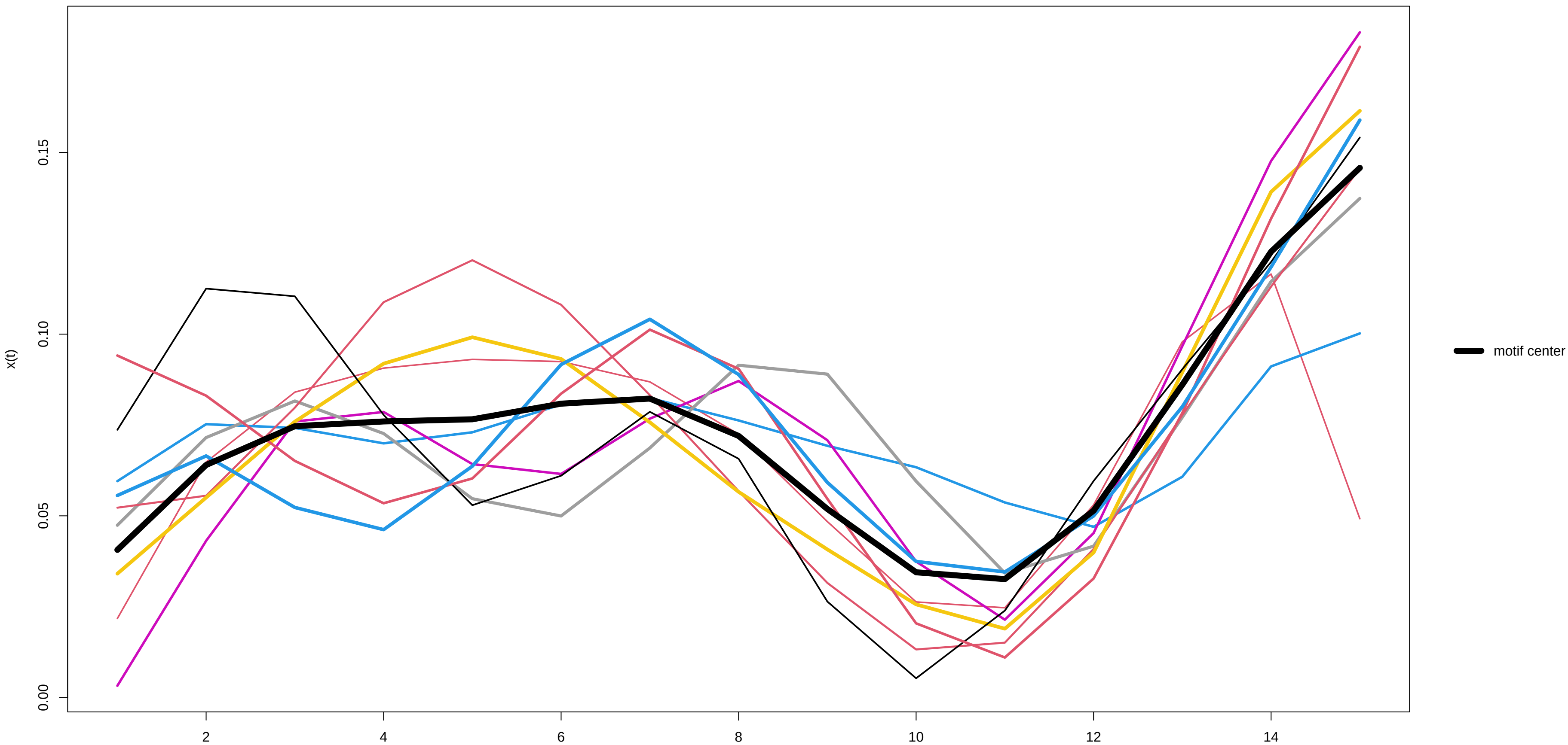
Motif 14 (9 occurrences) – x(t) derivative
