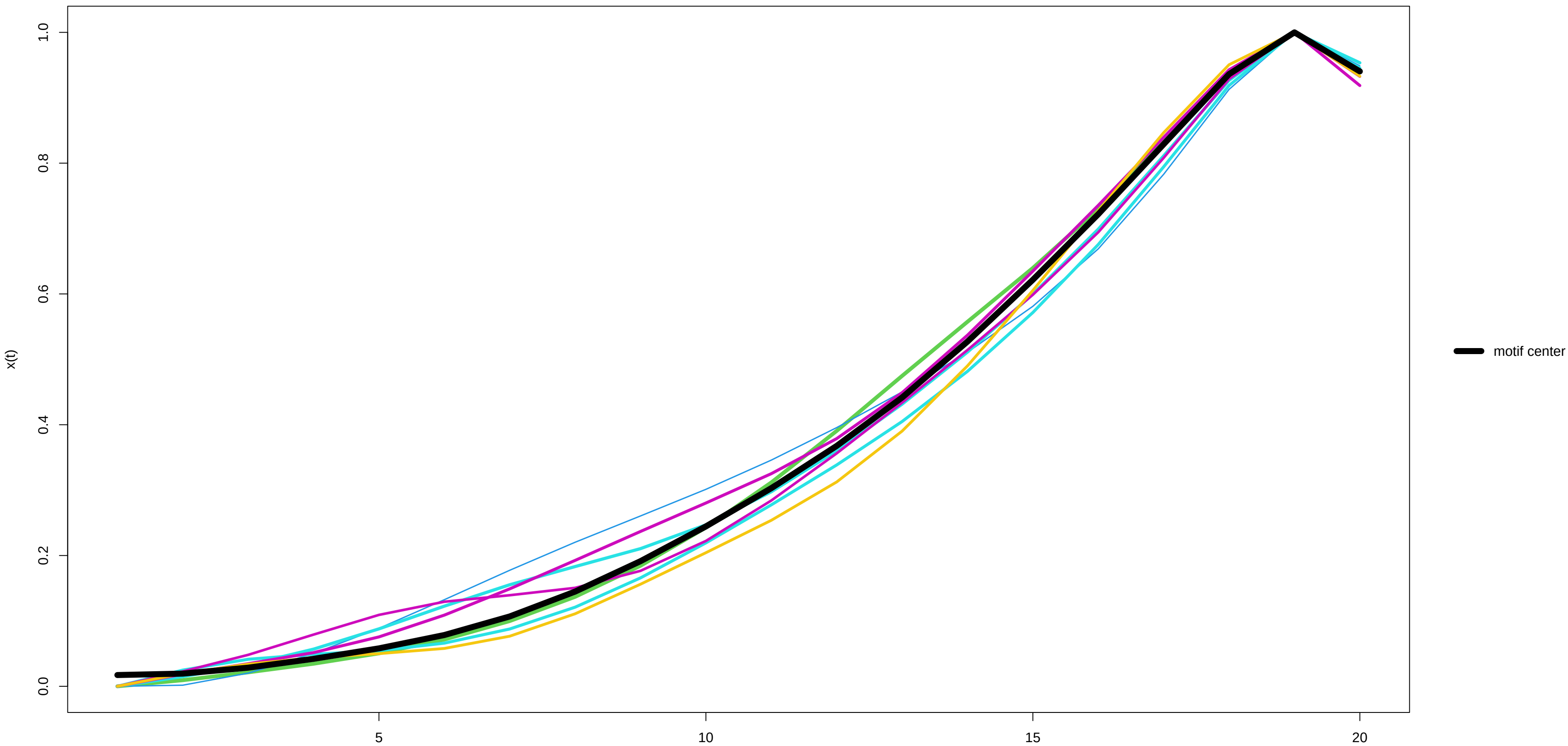
Motif 9 (7 occurrences) – x(t)
