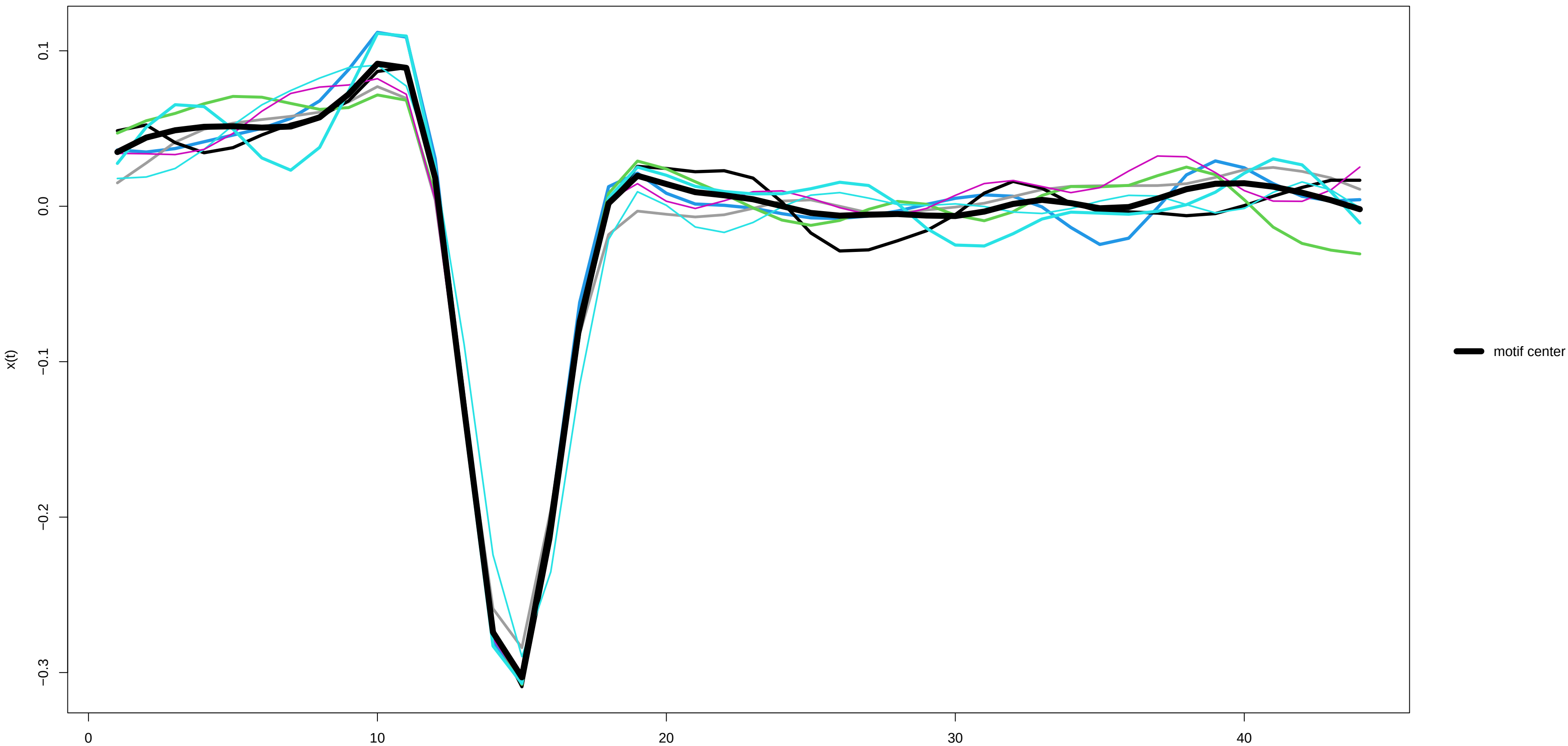
Motif 12 (7 occurrences) – x(t) derivative
