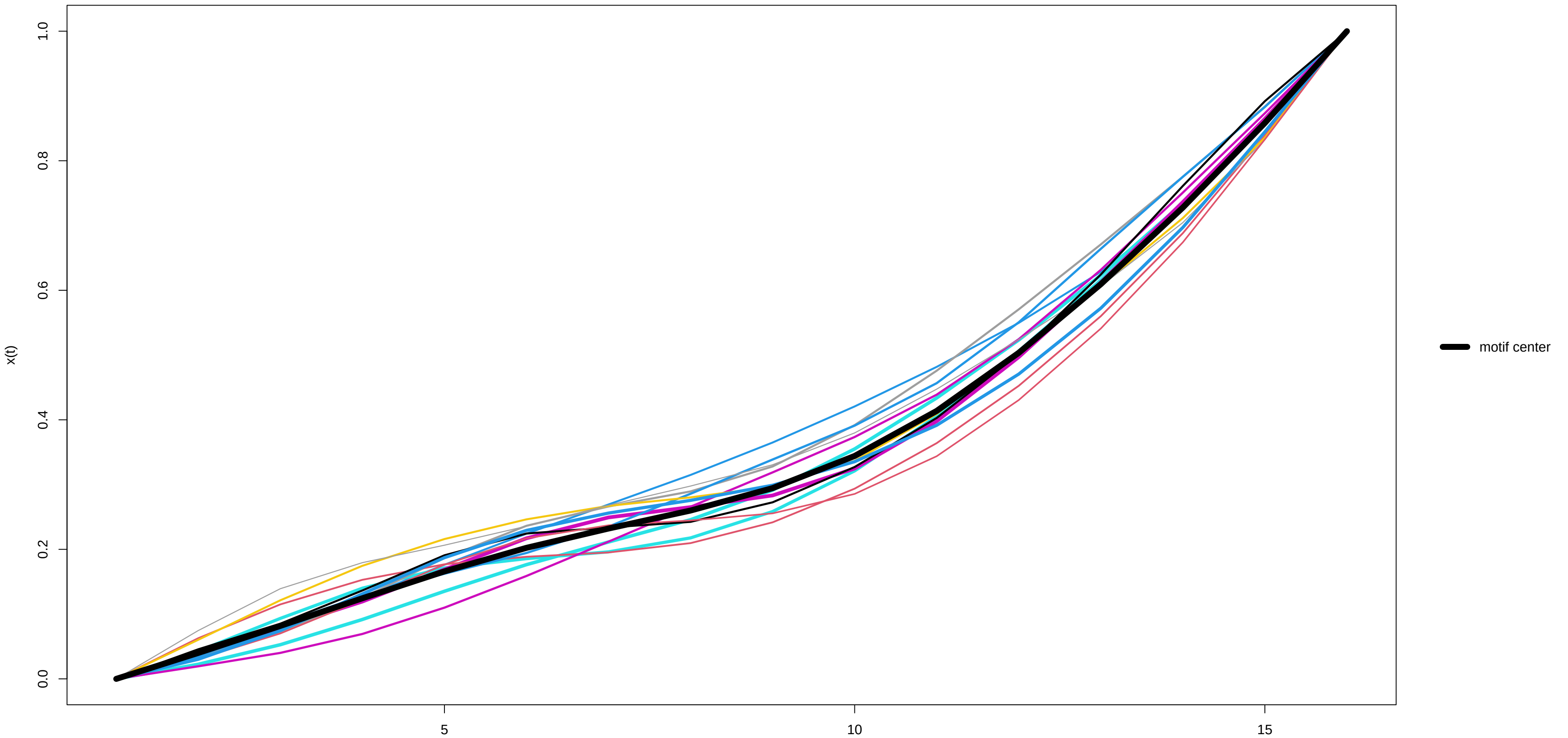
Motif 3 (13 occurrences) – x(t)
