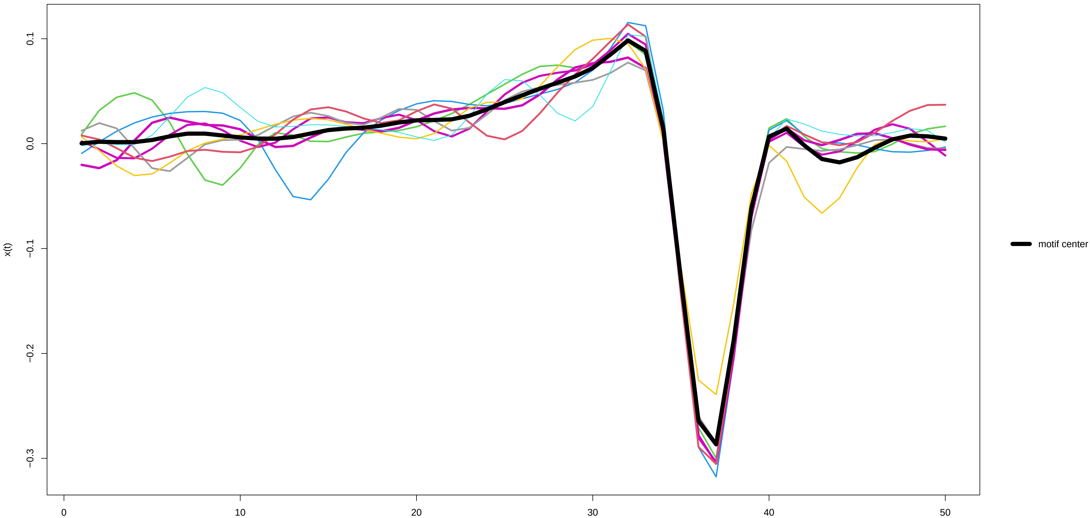
Motif 16 (8 occurrences) – x(t) derivative
