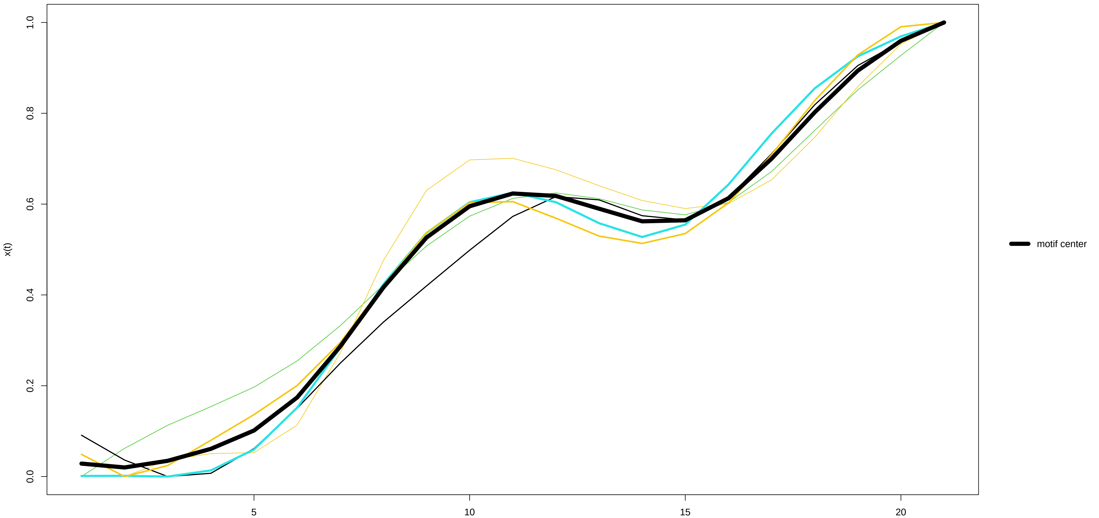
Motif 18 (5 occurrences) – x(t)
