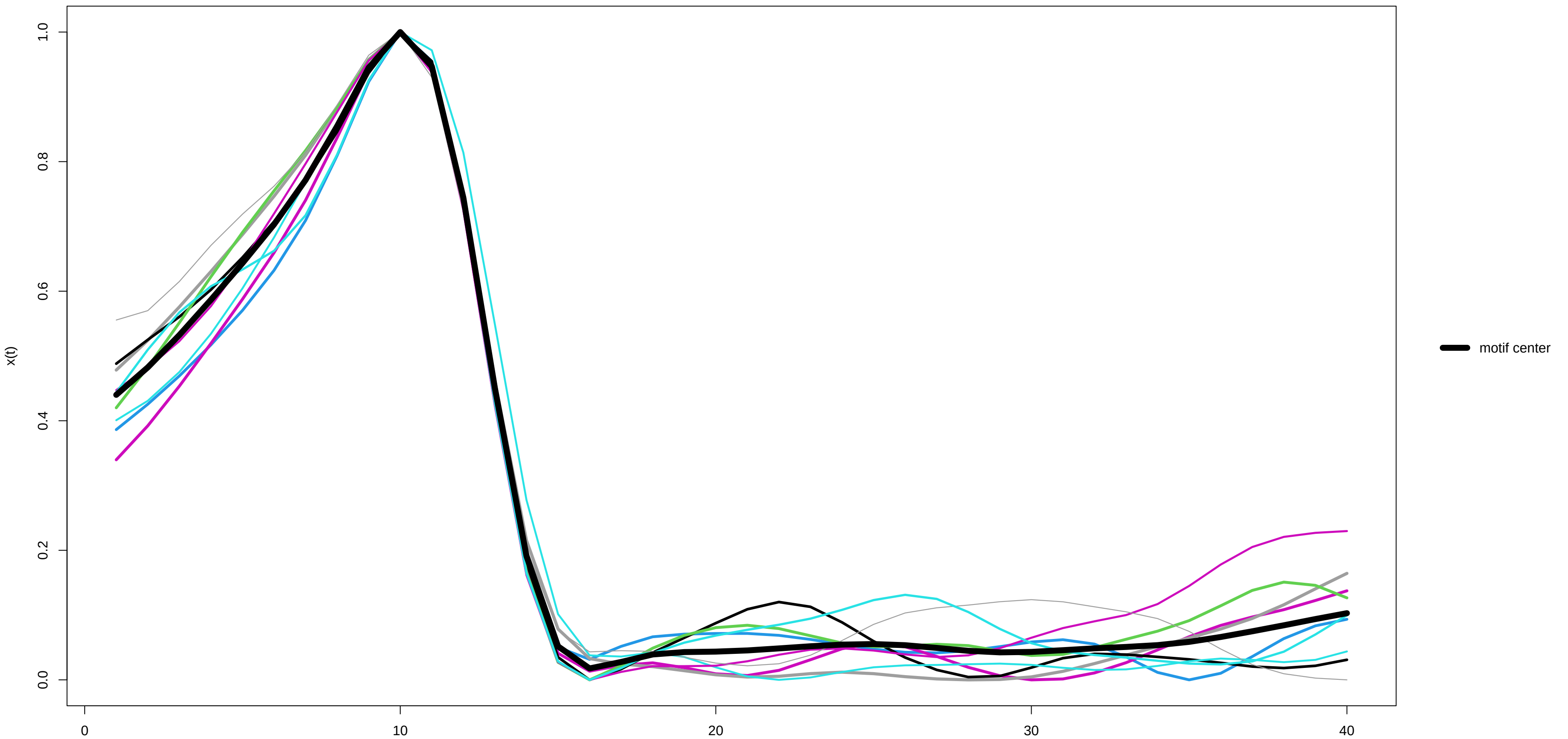
Motif 8 (9 occurrences) – x(t)
