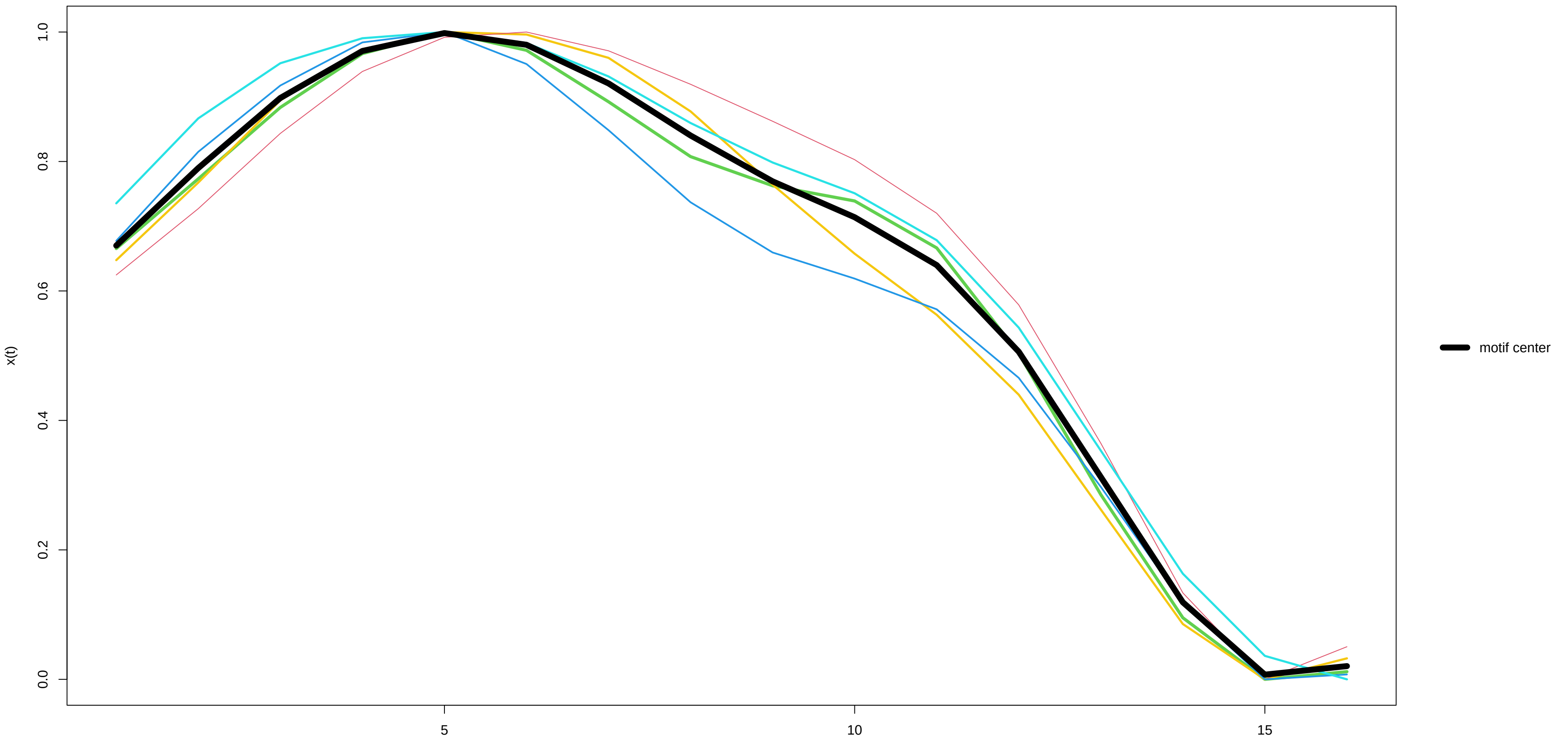
Motif 17 (5 occurrences) - x(t)
