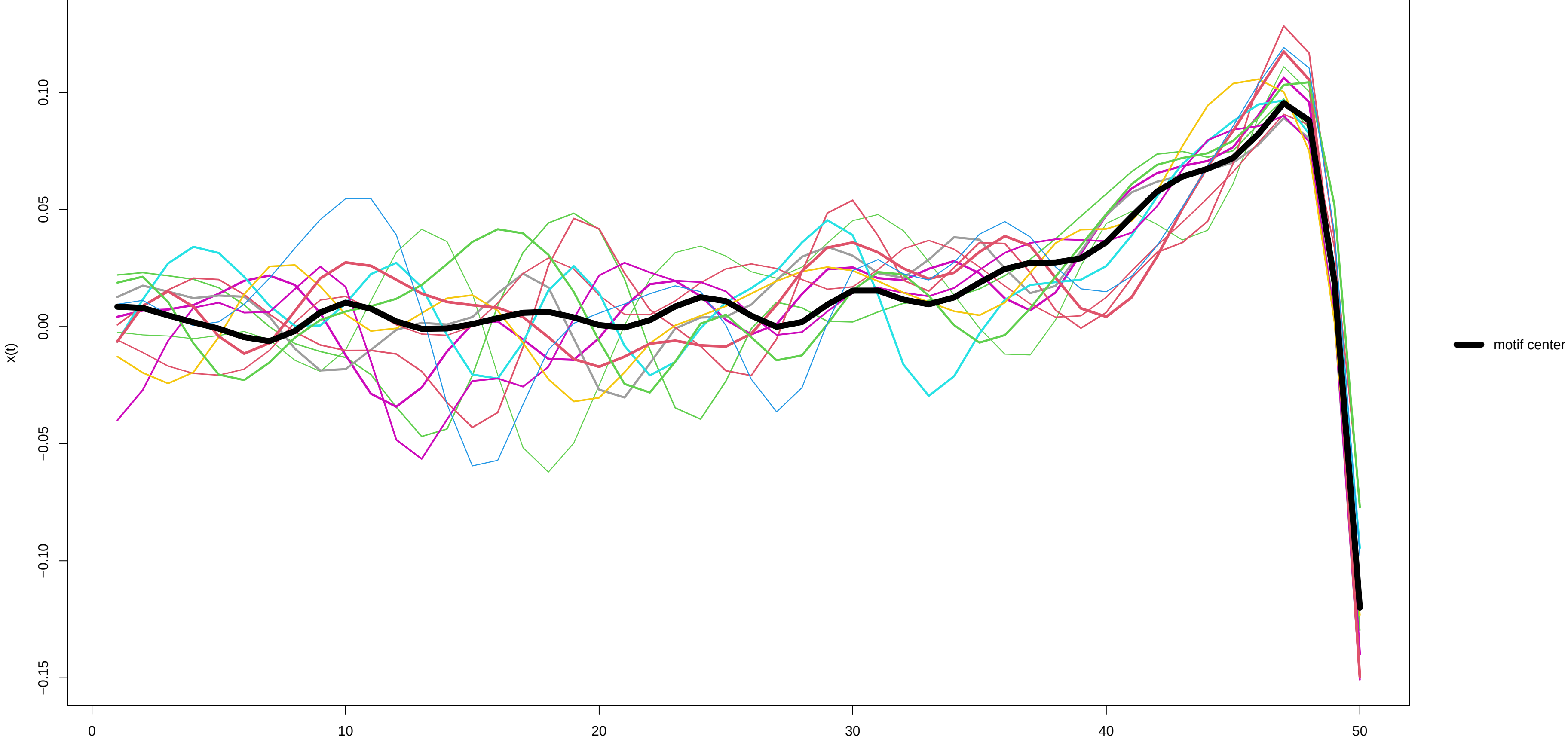
Motif 15 (12 occurrences) – x(t) derivative
