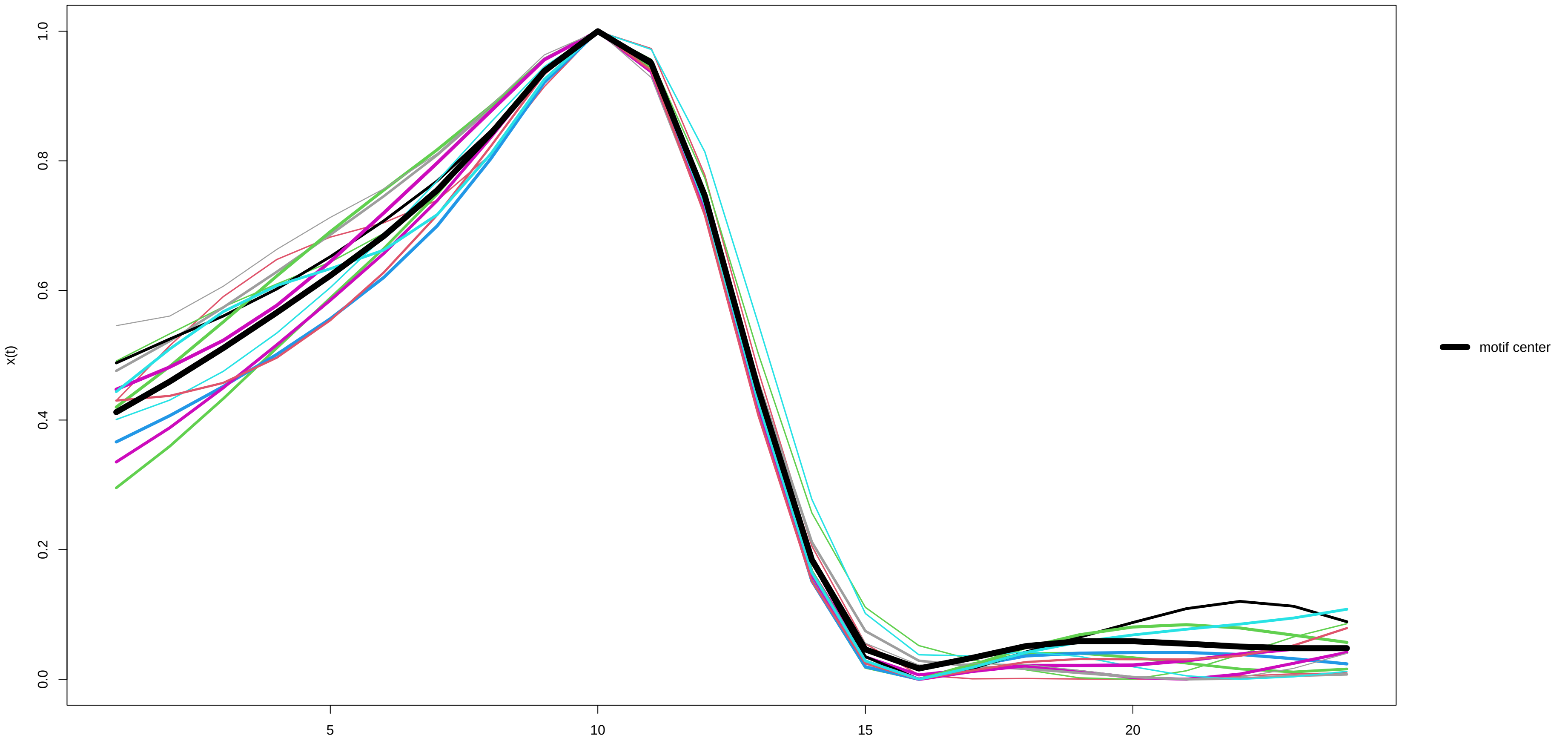
Motif 7 (13 occurrences) – x(t)
