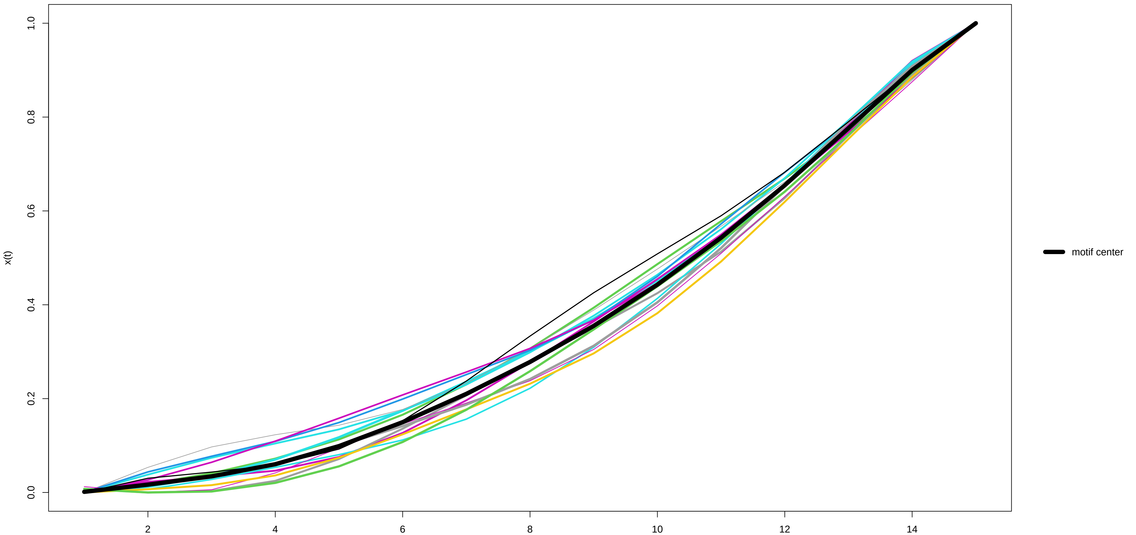
Motif 2 (14 occurrences) – x(t)
