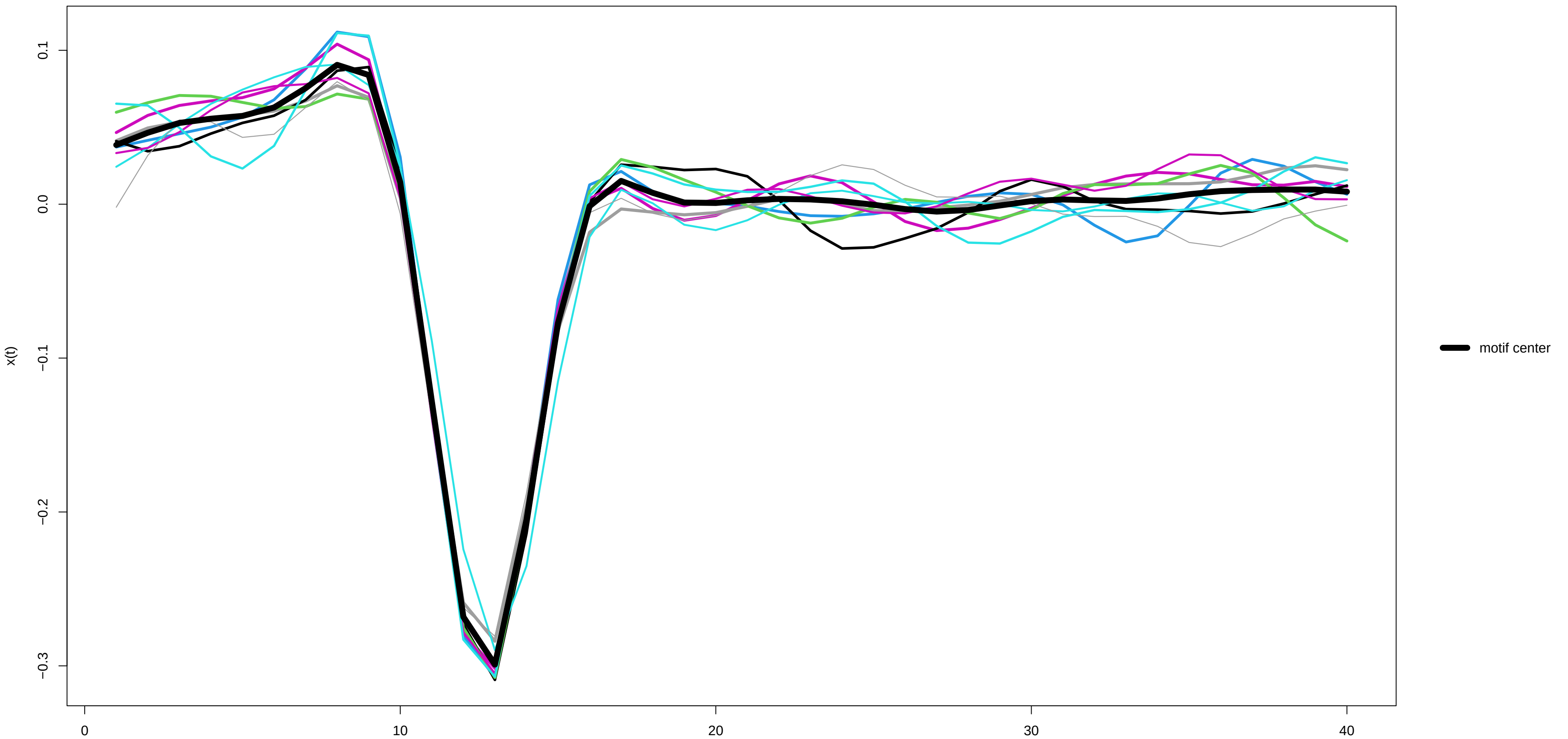
Motif 8 (9 occurrences) – x(t) derivative
