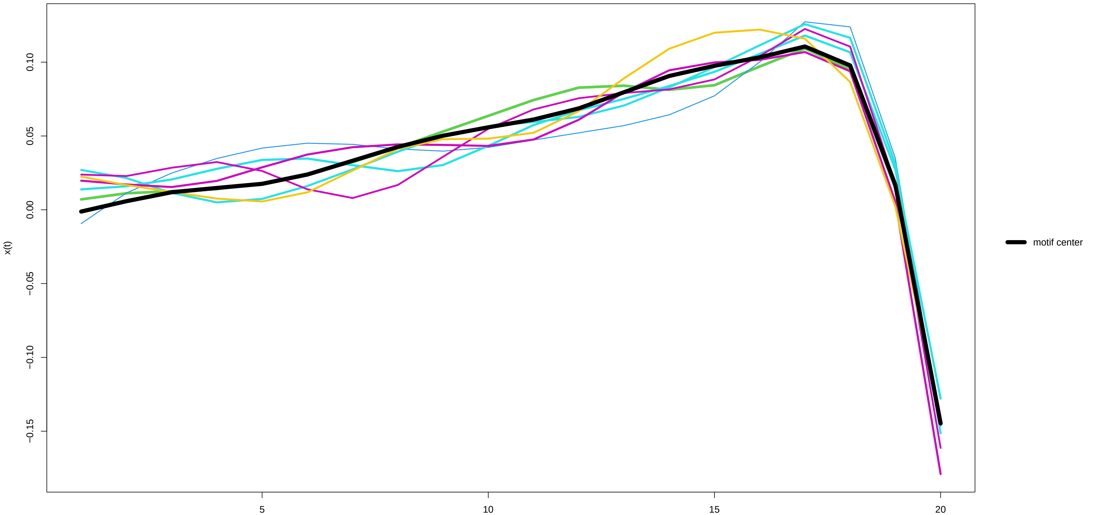
Motif 9 (7 occurrences) – x(t) derivative
