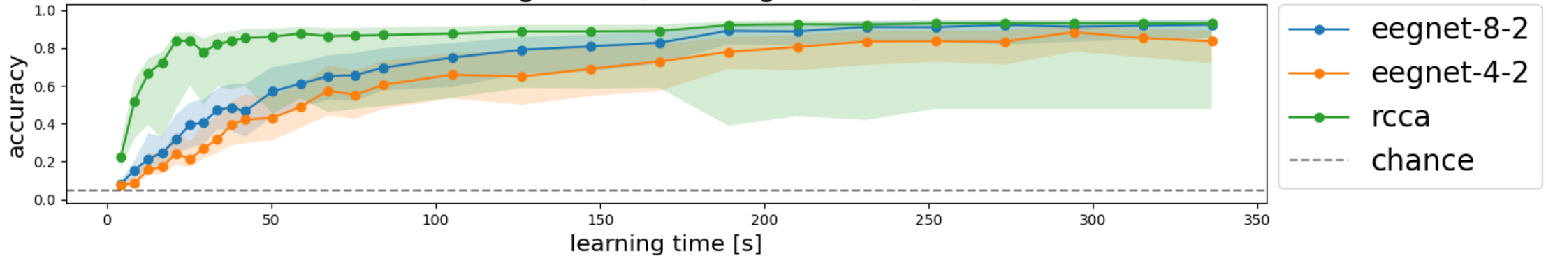
Learning curve (trial length = 4.2s)
