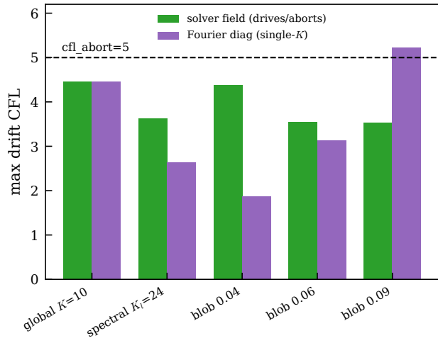
(b) real solver CFL vs Fourier diagnostic
