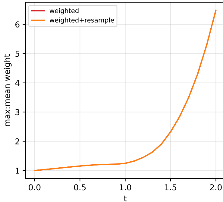
weight concentration
