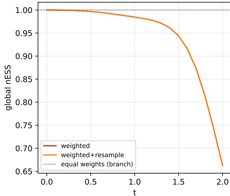
weight degeneracy
