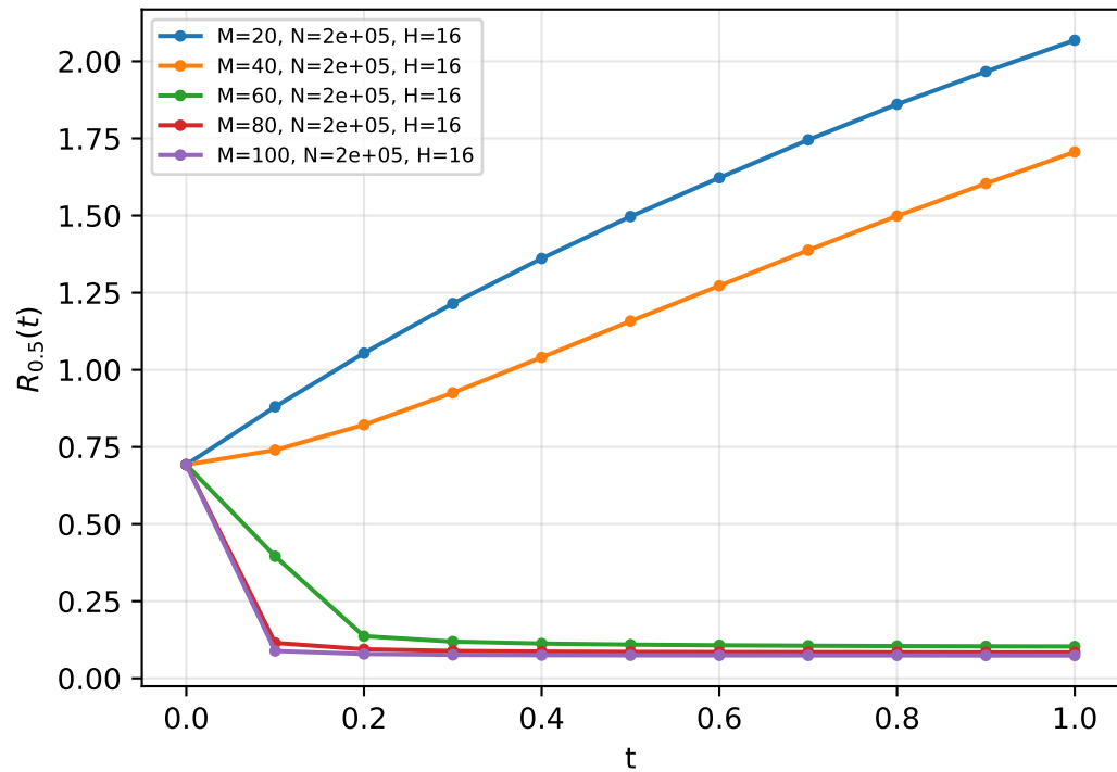
Inner half-mass core radius
