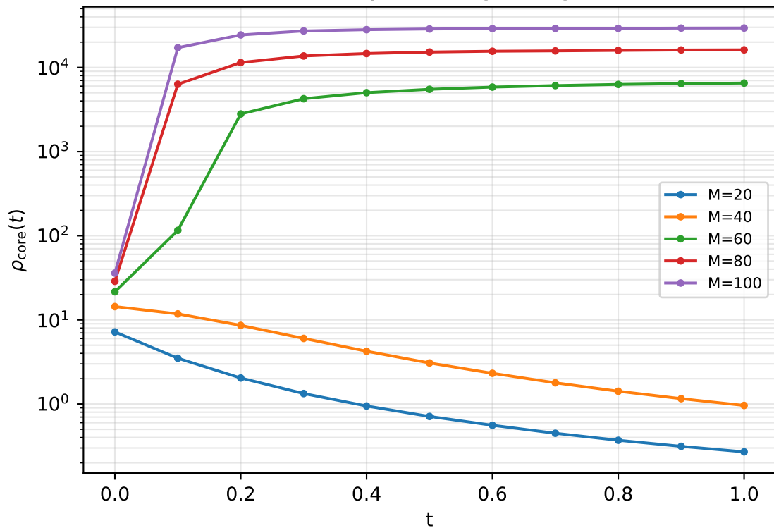
Core density (focusing surrogate)
