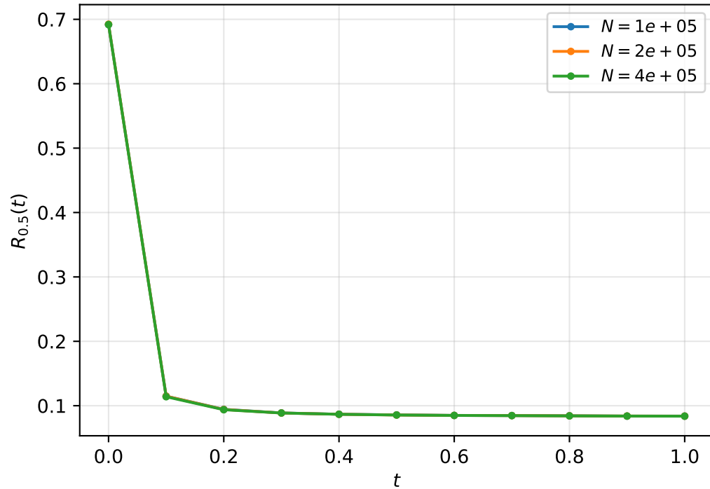
Core radius: particle-number convergence ( H = 16 )
