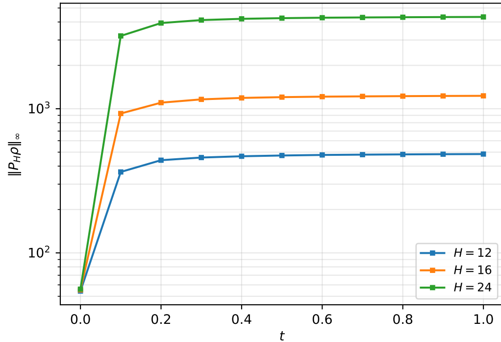
Reconstructed peak: bandwidth growth ( N = 10^5 )
