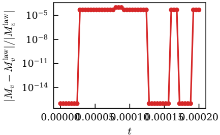
M_v law rel. err (max = 1.00e-04 )
