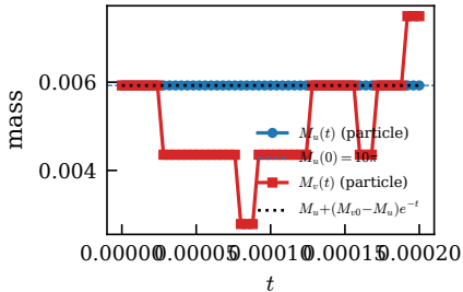
Mass conservation + chemical mass law +3.141e1
