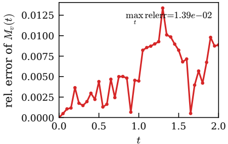
Injection-reaction unbiasedness
