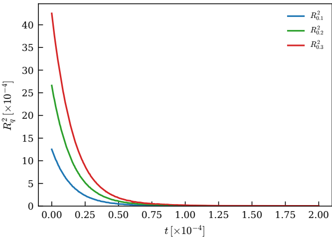
(a) R_q^2(t) + linear fits (LDG N=320)
