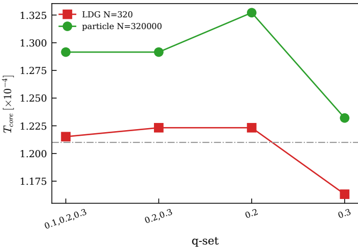
(e) q-set sensitivity
