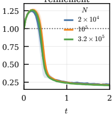
(b) Particle-number refinement
