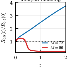
(a) Diffusion and delayed focusing
