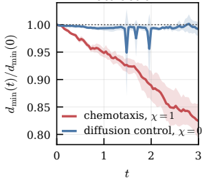
(b) Inter-cluster attraction
