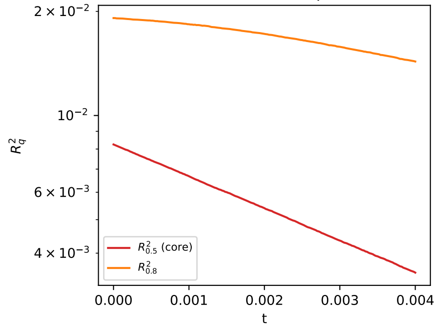
core radius collapse
