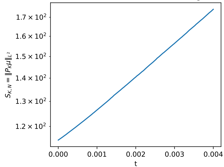
reconstructed L2 norm (focusing)
