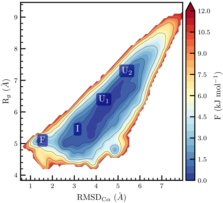
(a) FES: \text{RMSD}_{\text{C}\alpha} vs R_g
