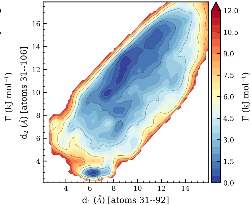
(c) FES: cross-strand contact distances
