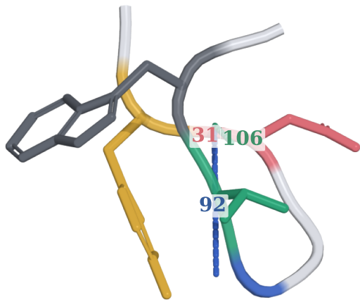
(a) Native contact definitions
