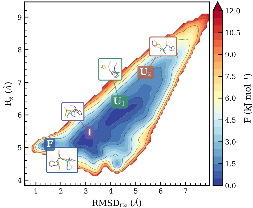
(b) FES: \text{RMSD}_{\text{C}\alpha} vs R_g
