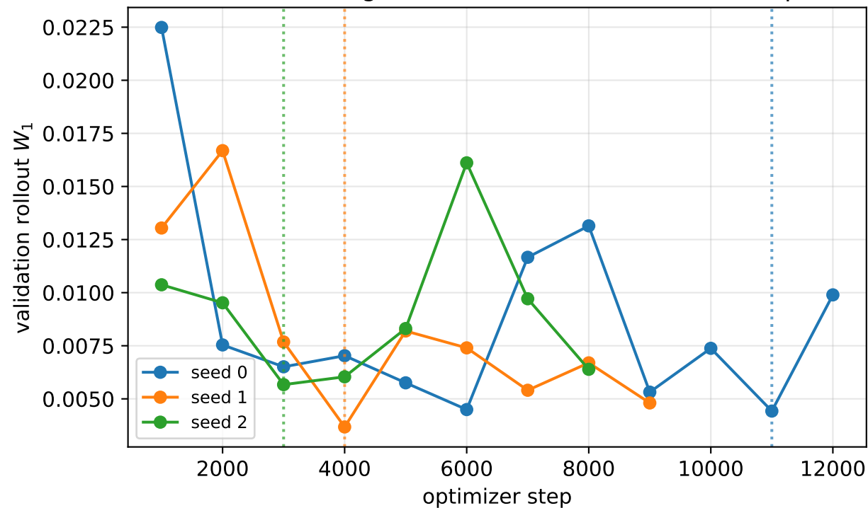
MVNN learning curves (final); dotted = best step
