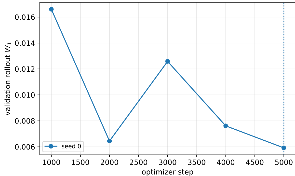
MVNN learning curves (pilot); dotted = best step
