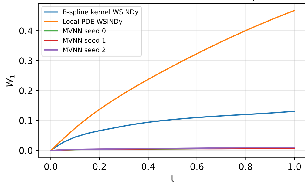
Mean W_1(t) across confirmation triplets
