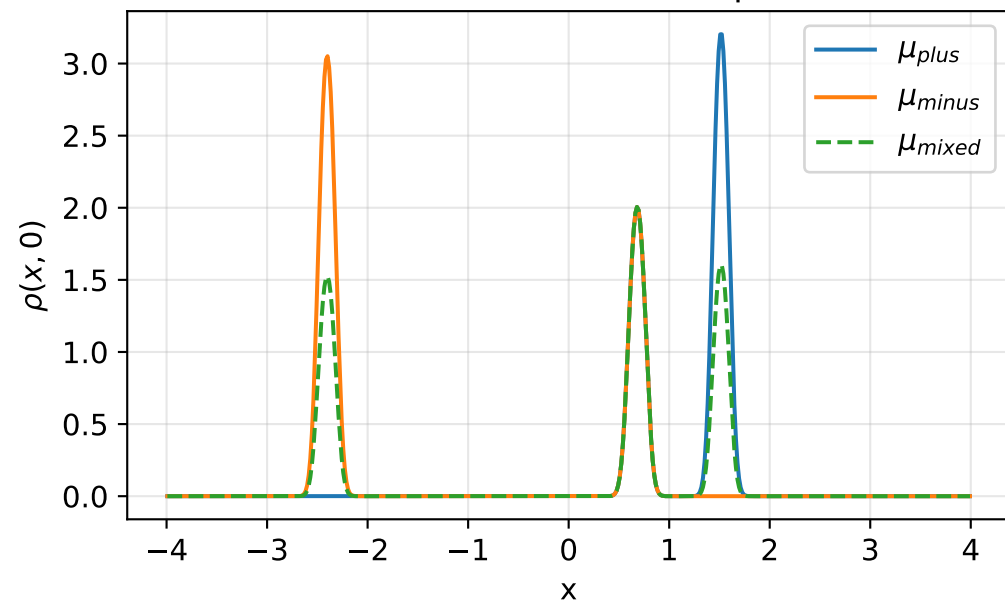
Matched initial densities (triplet 100)
