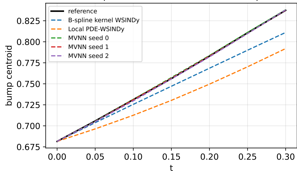
Central-bump centroid, mixed measure (triplet 100)
