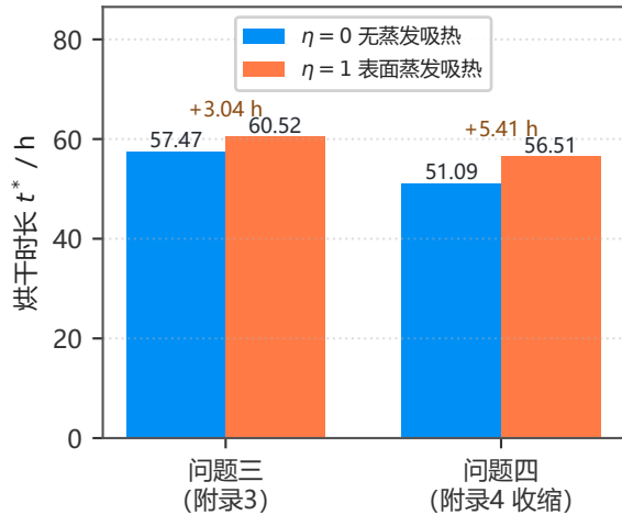
(b) 烘干时长对照
