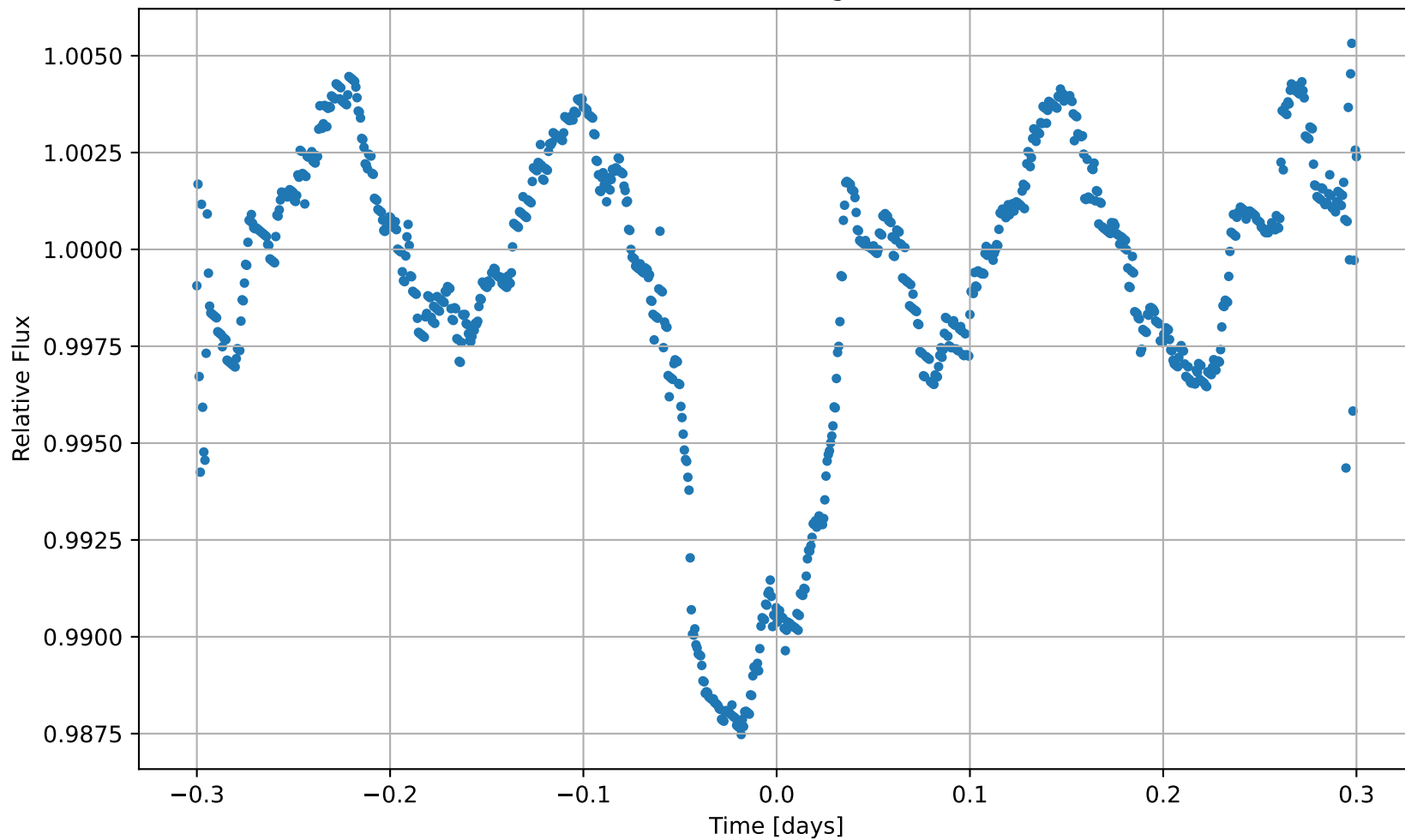
Part 3: Cleaned Light Curve
