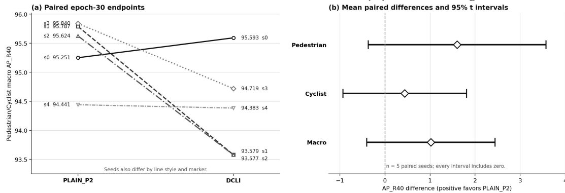
Figure 2. Five-seed terminal evidence. (a) Each line links the two methods for one registered seed. (b) Points are paired means and bars are two-sided 95% t intervals. All intervals include zero; positive differences favor PLAIN_P2.
