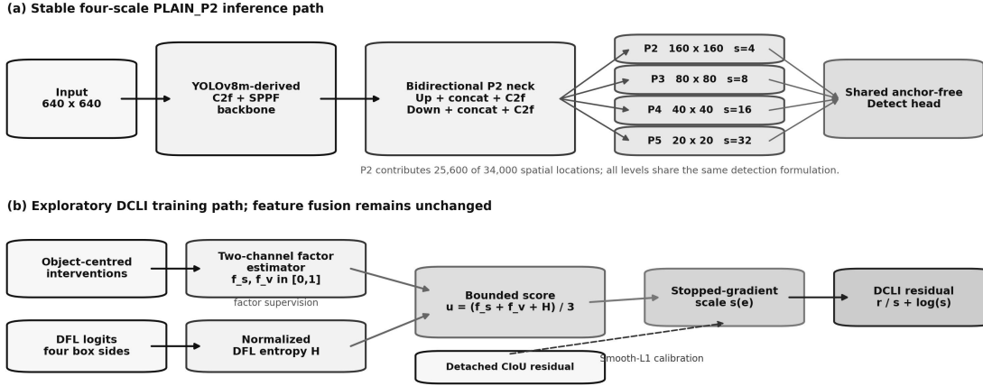
Figure 1. Method overview. (a) PLAIN_P2 is the stable inference path: a YOLOv8m-derived backbone feeds a bidirectional neck and a shared head at strides 4–32. (b) DCLI is an exploratory training path. Learned degradation factors and normalized DFL entropy define a bounded score; stopped-gradient conditioning prevents a shortcut through the box loss. Feature concatenation remains unchanged in the frozen comparison.
