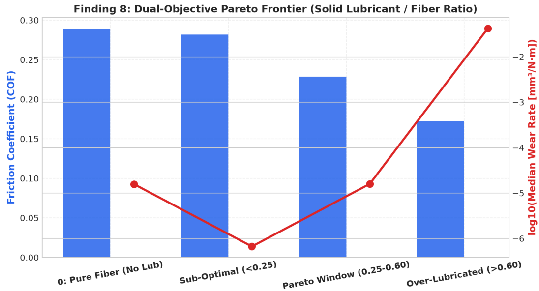
Figure 6.3: Finding 8 — Solid Lubricant to Fiber Reinforcement Pareto Window
