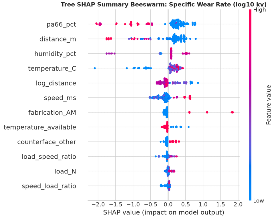
Figure 6.6: Global Tree SHAP Beeswarm Feature Impact Summary for Wear Rate
