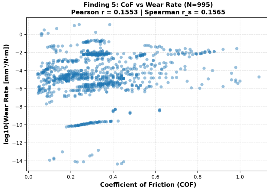
Figure 6.4: Finding 5 — Orthogonality Scatter Plot of CoF versus Specific Wear Rate
