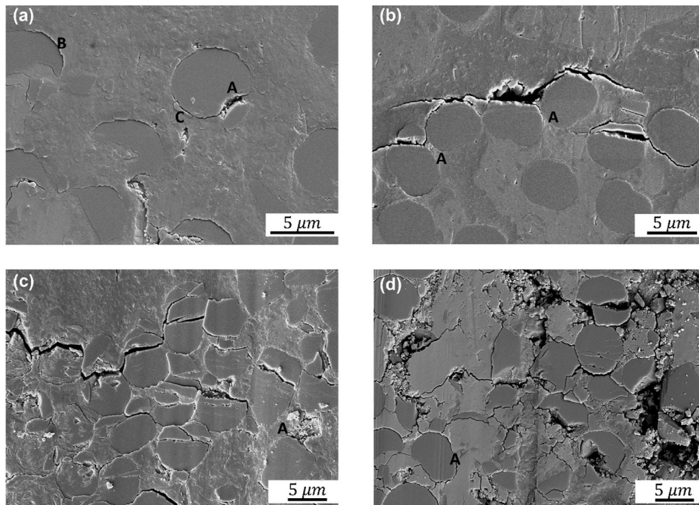
Fig. 9. Worn surfaces of specimens in N fibre orientation with different testing durations: (a) 1h; (b) 3h; (c) 5h; (d) 10h.
