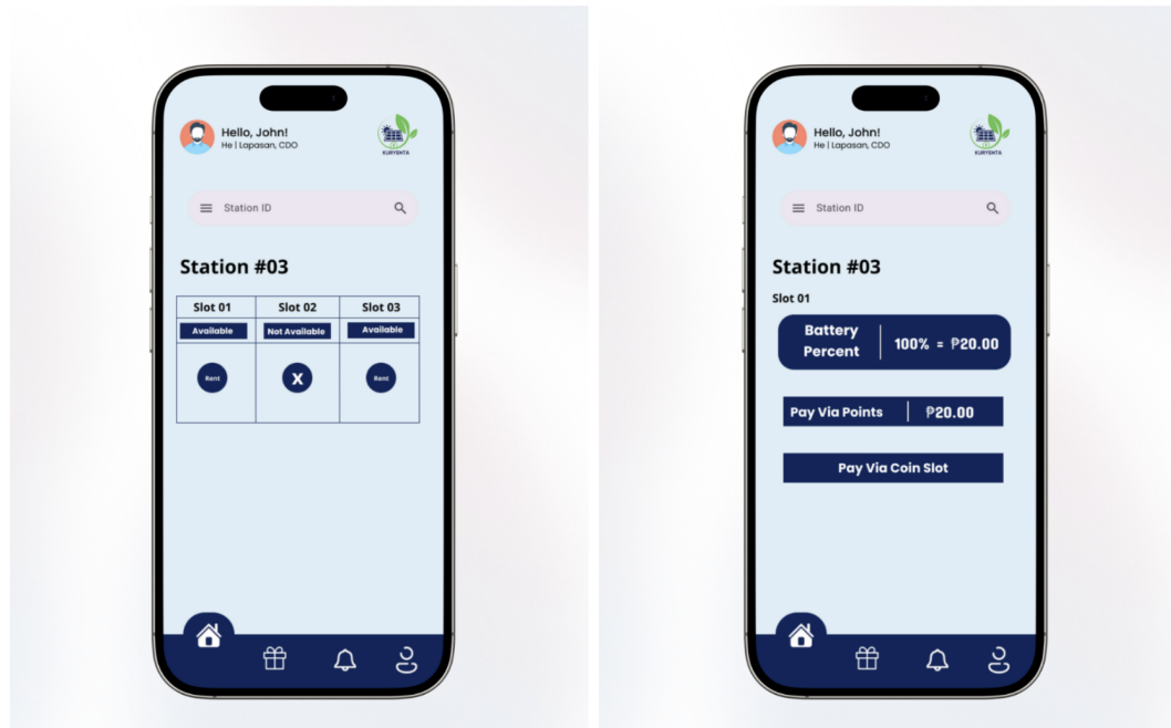
Figure 3.20 Renting Screen
