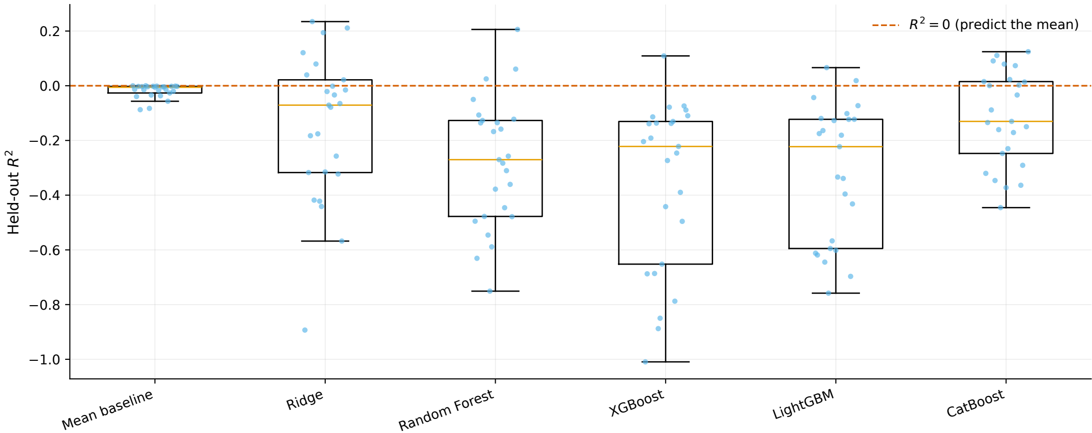
Participant-grouped 5-fold CV x 5 repeats (25 folds)
