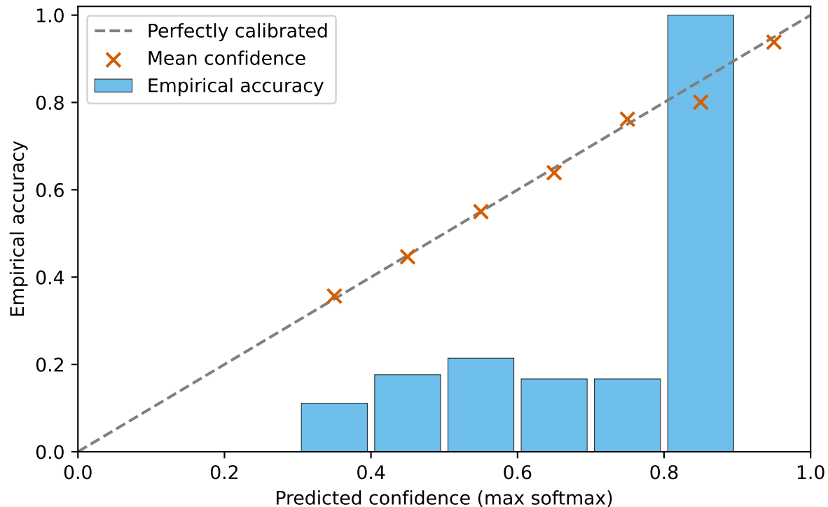
Reliability diagram - ECE = 0.253
