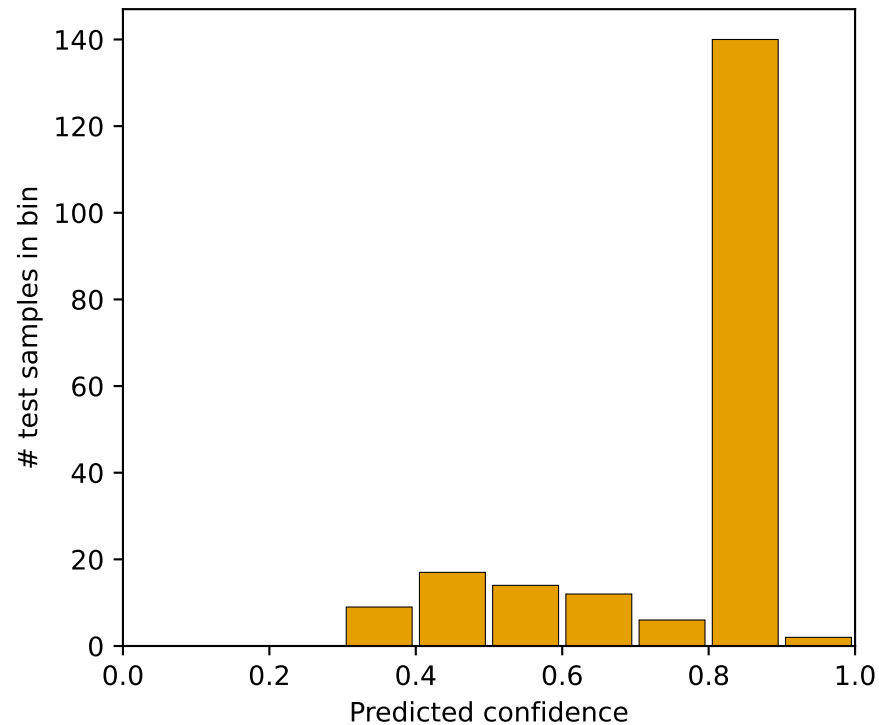
Confidence histogram
