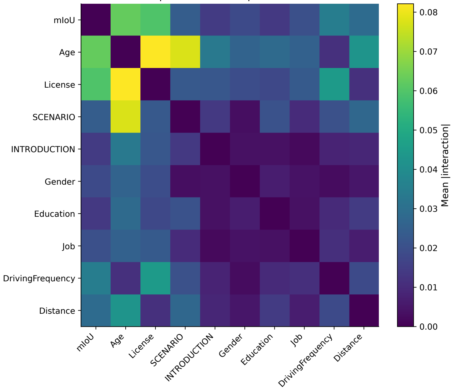
Mean |SHAP interaction| across features
