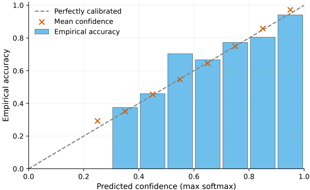
Reliability diagram - ECE = 0.055
