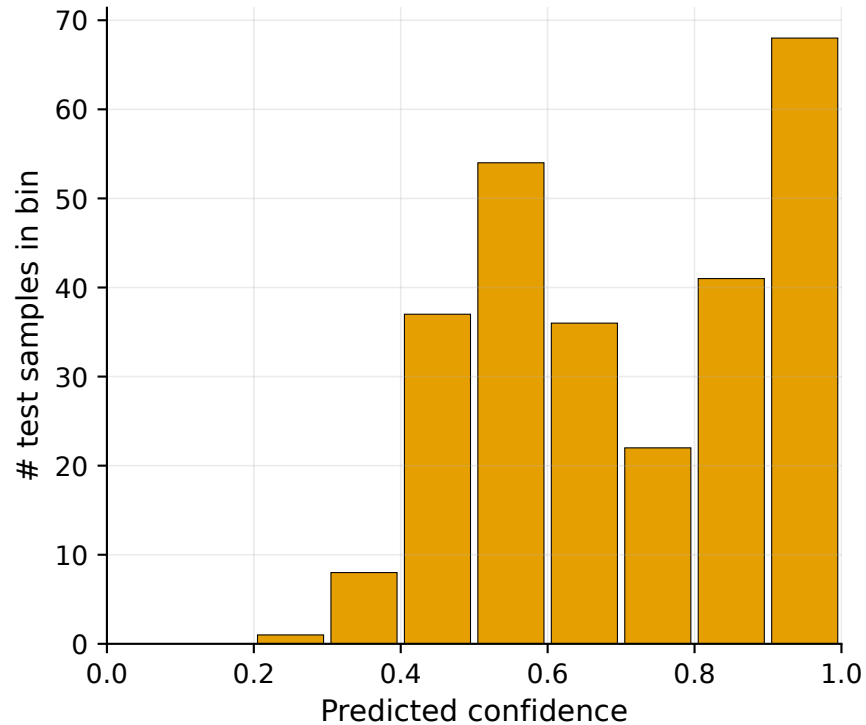
Confidence histogram
