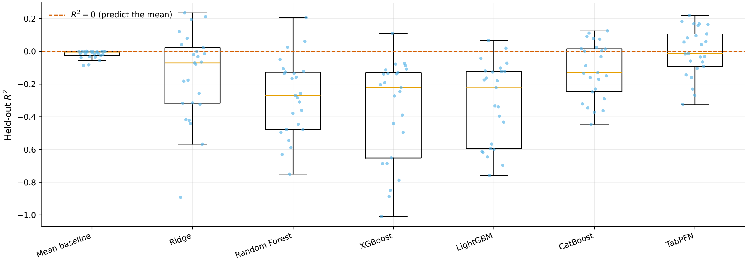
Participant-grouped 5-fold CV x 5 repeats (25 folds)
