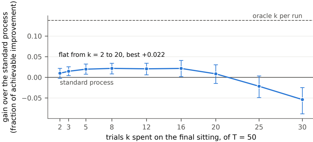
Figure 3: Gain over the standard process from spending the last k of T = 50 trials on one comparative sitting among the top- k visited designs, in units of the achievable improvement, with 95% landscape-bootstrap intervals. The dashed line is the hindsight-best k per run. Pooled over the four error processes, all four magnitudes and both onsets, with LogEI and qNEI. The looks carry the full idiosyncratic SD.
