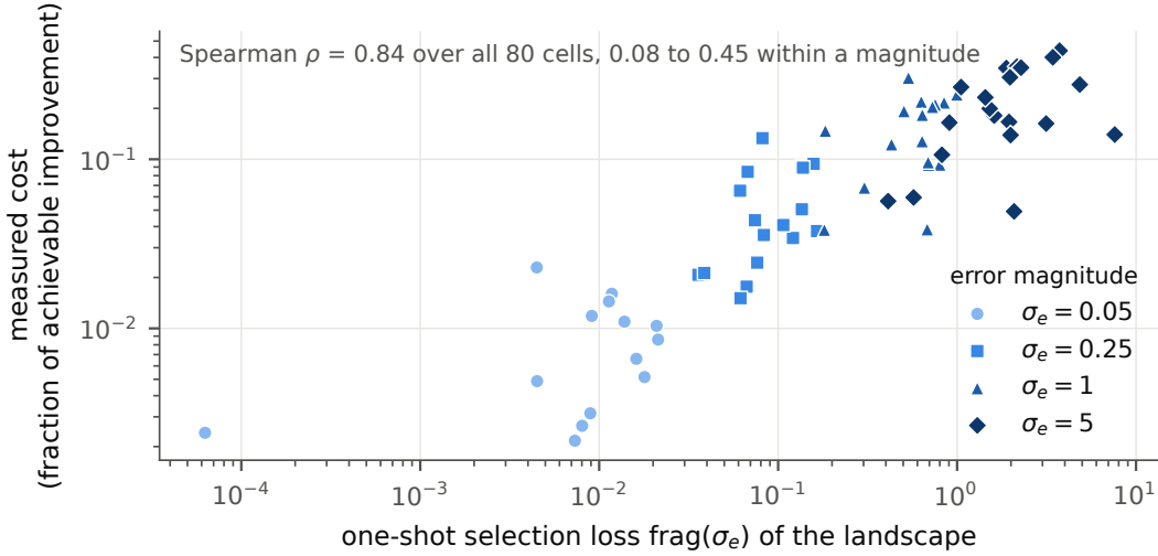
Figure 4: The one-shot selection loss \text{frag}(\sigma_e) of a landscape (Equation 6, computed on 256 quasi-random designs with no optimizer) against the trajectory cost the sweep measured on it, one point per landscape and magnitude, error from the first rating. Shape and shade both encode the magnitude. Nine of the eighty cells cannot be placed on log axes, eight because frag is exactly zero and one because the measured cost is negative. Both correlations in the panel are over all eighty. The pooled value largely restates that both quantities grow with \sigma_e , which is why the within-magnitude range is given beside it.
