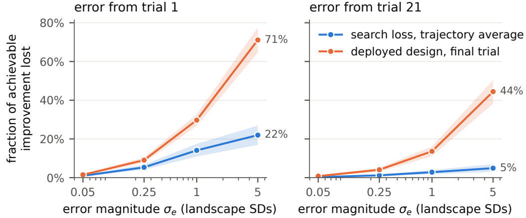
Figure 1: The two responses against the error magnitude, from Table 1: the post-onset trajectory average of search loss and the deployed design’s loss at the final trial, as fractions of the achievable improvement, averaged over twenty landscapes and ten model-based acquisitions. Bands are 95% landscape bootstraps. The two are on different time bases, so their difference is not the selection loss of Section 5.
