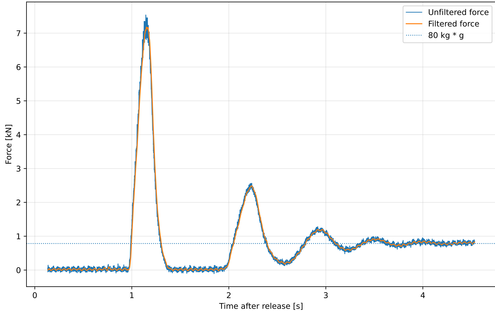
UIAA fall: force vs. time
