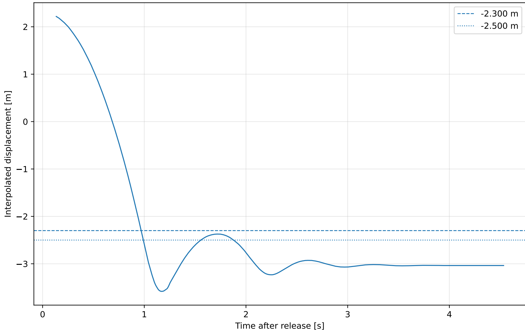
UIAA fall: displacement vs. time
