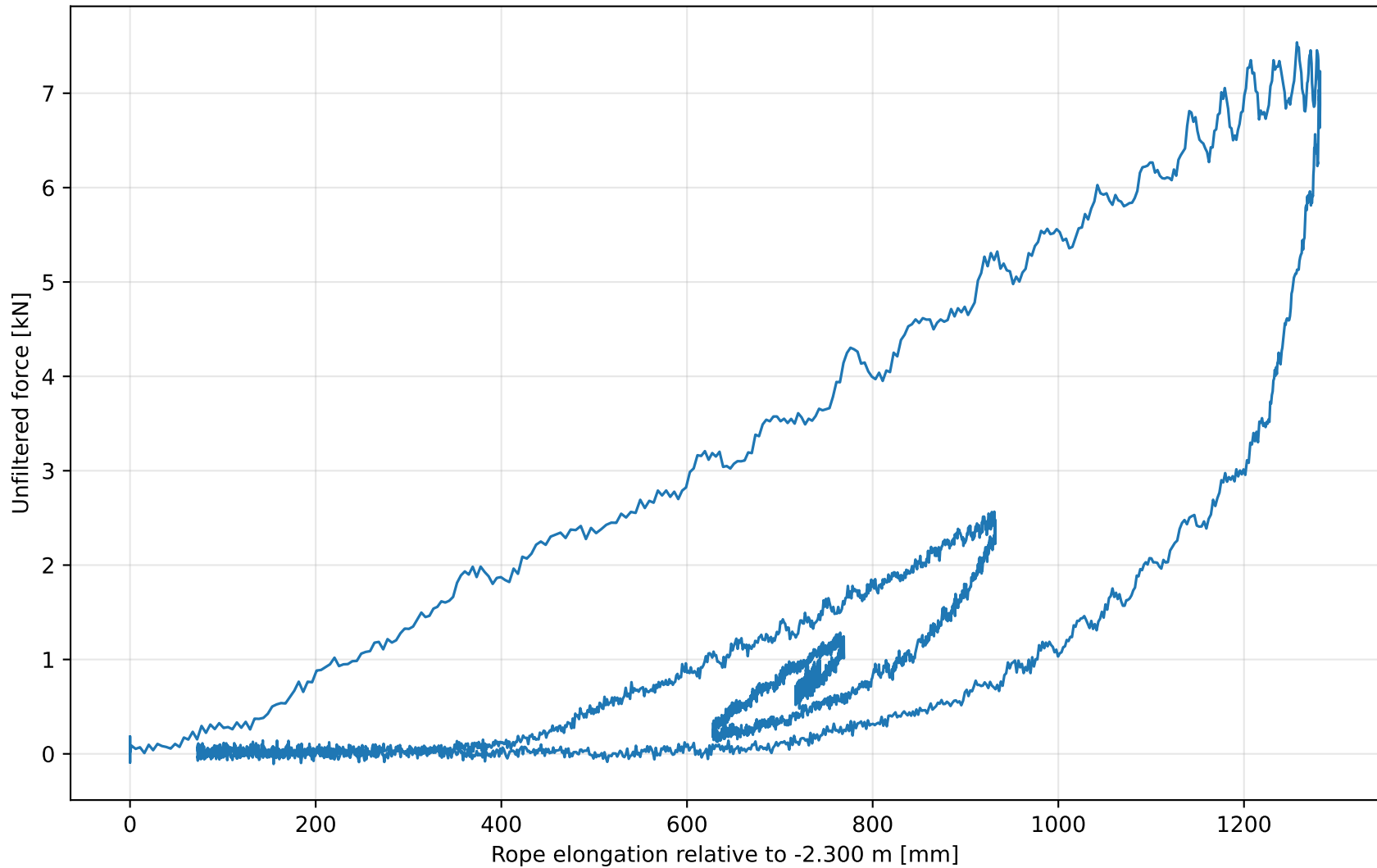
UIAA fall: unfiltered force vs. rope elongation
