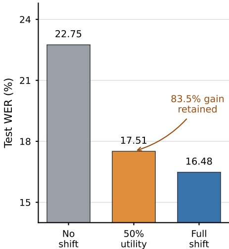
Same model, frozen CTC head
