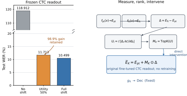
Fig. 1. DADS measures and intervenes on the fine-tuning shift. Paired representations yield \Delta = E_{\text{ft}} - E_{\text{pt}} ; Taylor utility ranks its coordinates; a retained mask is supplied to the original fine-tuned CTC readout. The left panel shows the official Fold 0 intervention at the 50% budget.
