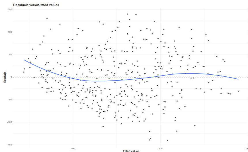
Figure 3: Residuals vs. Fitted Values diagnostic plot for the multiple linear regression model showing homoscedastic error distribution.
