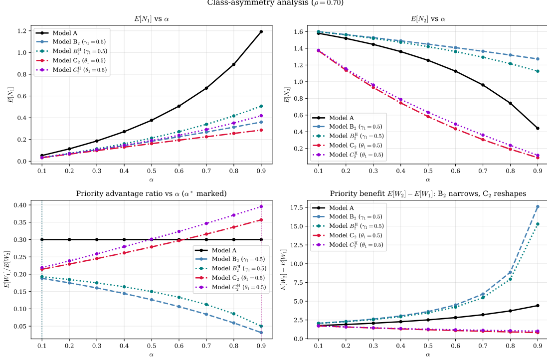
Figure 23: Class-asymmetry sweep at \rho = 0.70 : E[N_1] , E[N_2] , the priority ratio E[W_1]/E[W_2] (vertical dotted lines mark each model's ratio-extremising split over the swept range [0.1, 0.9] ), and the absolute priority benefit E[W_2] - E[W_1] , for Models A , B_2 and B_2^H ( \gamma_1 = 0.5 ), and C_2 and C_2^H ( \theta_1 = 0.5 ).
