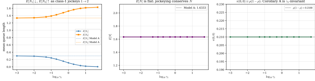
Figure 20: Model-B 2 at \rho = 0.70 ( \lambda_1 = 0.3 , \lambda_2 = 0.4 , \mu = 1 ). Left : \mathbb{E}[N_1] decreases and \mathbb{E}[N_2] increases monotonically in \gamma_1 (Model-A values dotted). Centre : \mathbb{E}[N] is flat — jockeying conserves the total count. Right : \pi(0,0) \equiv \rho(1-\rho) = 0.21 for all \gamma_1 , the numerical signature of Corollary 3.
