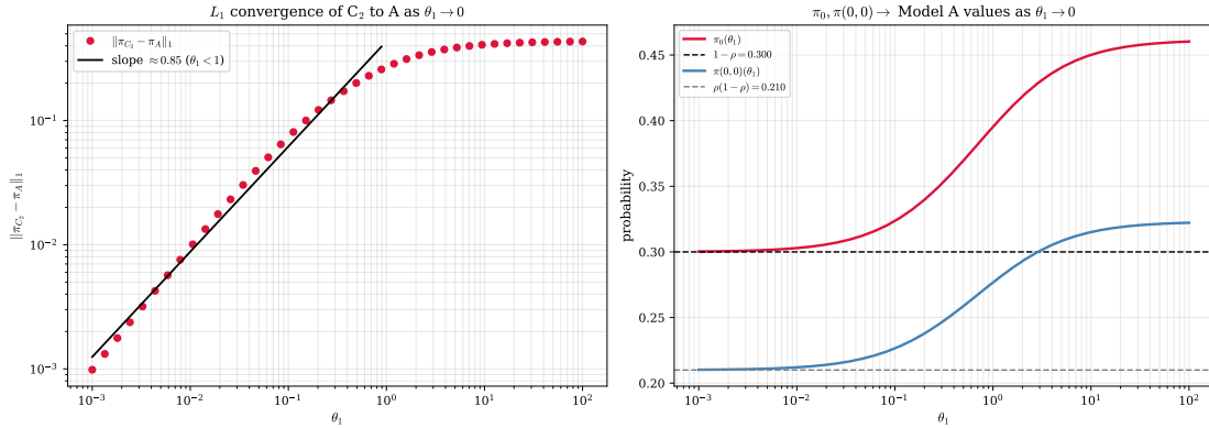
Figure 27: Convergence of Model- C_2 to Model-A as \theta_1 \rightarrow 0^+ ( \lambda_1 = 0.3 , \lambda_2 = 0.4 , \mu = 1 ). Left : log–log plot of \|\pi_{C_2} - \pi_A\|_1 against \theta_1 , with a fitted slope of 0.85 over \theta_1 < 1 . Right : \pi_0(\theta_1) and \pi(0, 0)(\theta_1) relaxing onto the Model-A values 1 - \rho = 0.30 and \rho(1 - \rho) = 0.21 as \theta_1 \rightarrow 0 .
