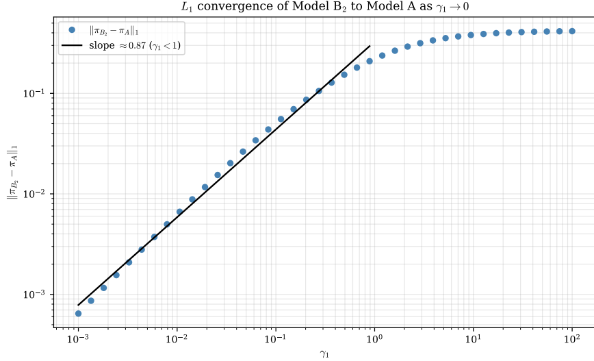
Figure 29: Convergence of Model- B_2 to Model-A as \gamma_1 \rightarrow 0^+ . The log-log L_1 distance has fitted slope 0.87 over \gamma_1 < 1 , again first-order, even though the B_2 limit is singular in the ODE (the \gamma_1 \rightarrow 0 limit is non-uniform in the analytic continuation, but the stationary distribution responds at first order).
