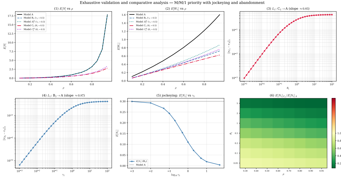
Figure 32: Synoptic dashboard of the numerical study: (1) E[N] and (2) E[W_1] versus \rho for all five solved models ( A , B_2 , B_2^H , C_2 , C_2^H ); (3) L_1 convergence C_2 \rightarrow A and (4) B_2 \rightarrow A ; (5) the jockeying effect on E[N_1] ; and (6) the E[N_1]_{C_2}/E[N_1]_A heatmap over (\rho, \theta_1) . Together these panels summarise the two central findings: jockeying redistributes delay at fixed total work, while abandonment reduces total work at a throughput cost.
