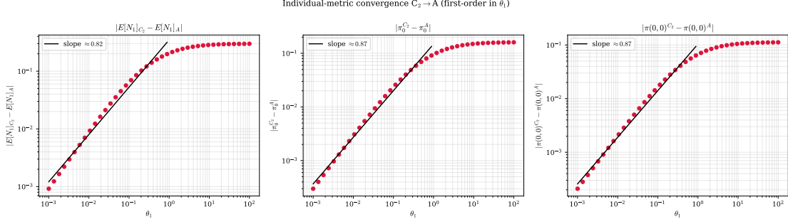
Figure 28: Individual-descriptor convergence of C_2 \rightarrow A : |\mathbb{E}[N_1]_{C_2} - \mathbb{E}[N_1]_A| , |\pi_0^{C_2} - \pi_0^A| and |\pi(0,0)^{C_2} - \pi(0,0)^A| versus \theta_1 on log-log axes, each annotated with its fitted slope.
