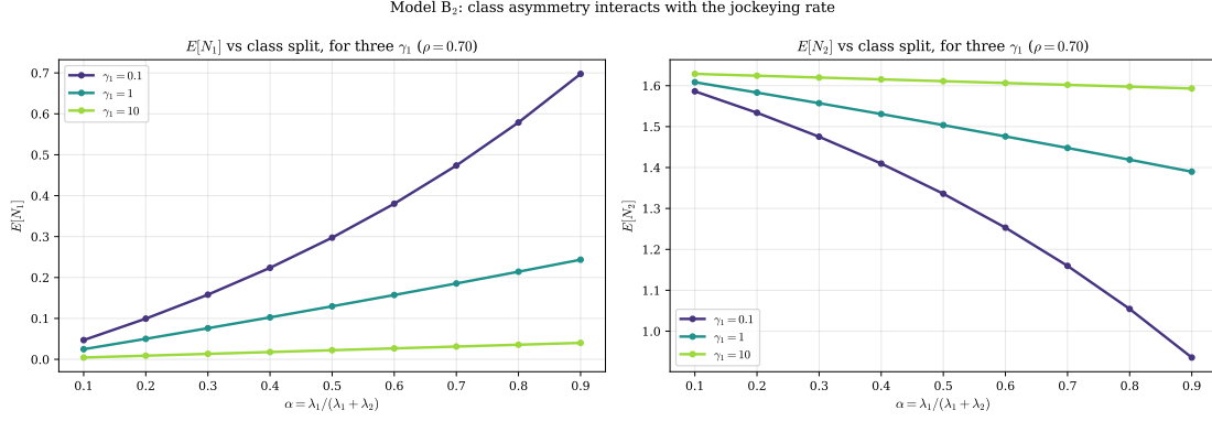
Figure 23: Model- B_2 : \mathbb{E}[N_1] and \mathbb{E}[N_2] versus the split \alpha for three jockeying rates \gamma_1 \in \{0.1, 1.0, 10.0\} at \rho = 0.70 . Stronger jockeying flattens \mathbb{E}[N_1] toward zero across the whole range of \alpha and loads the difference onto \mathbb{E}[N_2] .
