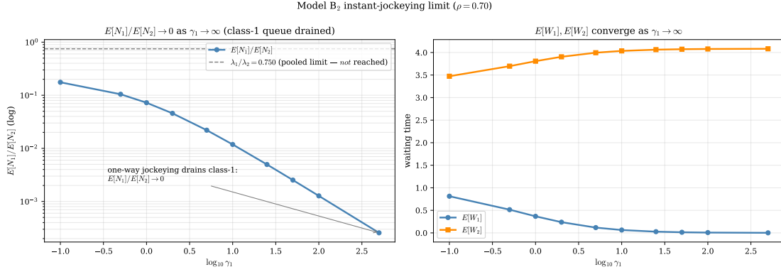
Figure 30: Model- B_2 in the strong-jockeying regime \gamma_1 \rightarrow \infty at \rho = 0.70 . Left : \mathbb{E}[N_1]/\mathbb{E}[N_2] \rightarrow 0 (note the logarithmic ordinate): one-way jockeying is absorbing, so the class-1 queue is drained completely. Right : \mathbb{E}[W_1] \rightarrow 0 while \mathbb{E}[W_2] saturates as \mathbb{E}[N_2] \rightarrow \mathbb{E}[N]_A .
